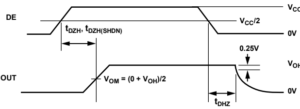
Figure 10. Driver Enable and Disable Times ( t_{DZH} , t_{DZH(SHDN)} , t_{DZH(SHDN)} )
