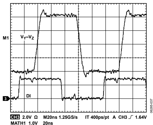
Figure 31. ADM3076E Driver Propagation Delay (16 Mbps)
