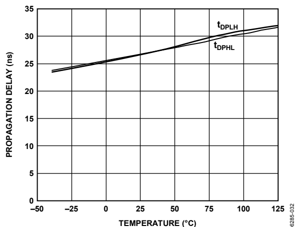
Figure 27. ADM3076E Driver Propagation Delay vs. Temperature (16 Mbps)
