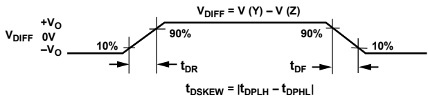
Figure 9. Driver Propagation Delays
