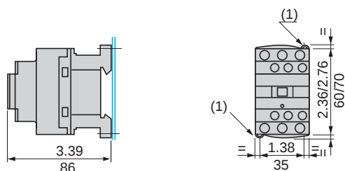
CAD (Vac Coil) Panel Mounted
