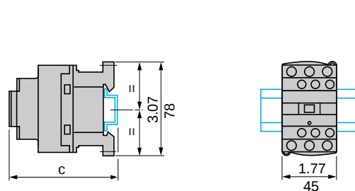
Mounted on AM1DP200 or DE200 Mounting Track
