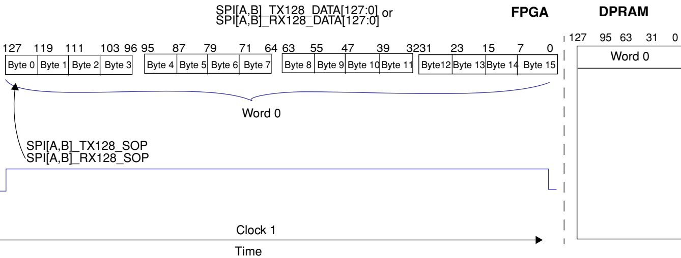
Figure 9. Byte and Bit Ordering in 128-Bit Mode
