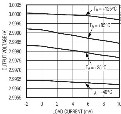
MAX6035 LOAD REGULATION ( V_{OUT} = 3V )
