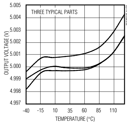
MAX6035AAUR50 OUTPUT VOLTAGE TEMPERATURE DRIFT
