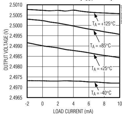
MAX6035 LOAD REGULATION ( V_{OUT} = 2.5V )
