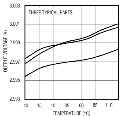
MAX6035AAUR30 OUTPUT VOLTAGE TEMPERATURE DRIFT
