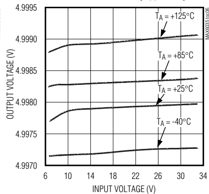
MAX6035 LINE REGULATION ( V_{OUT} = 5V )
