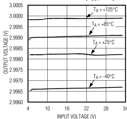
MAX6035 LINE REGULATION ( V_{OUT} = 3V )
