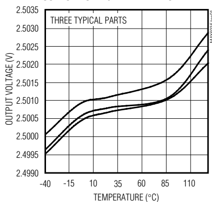
MAX6035AAUR25 OUTPUT VOLTAGE TEMPERATURE DRIFT
