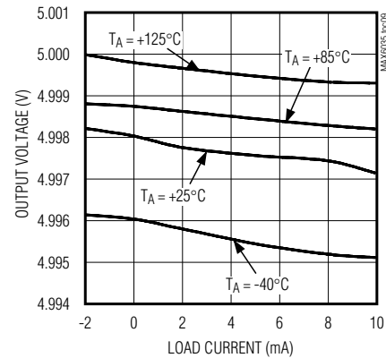
MAX6035 LOAD REGULATION ( V_{OUT} = 5V )
