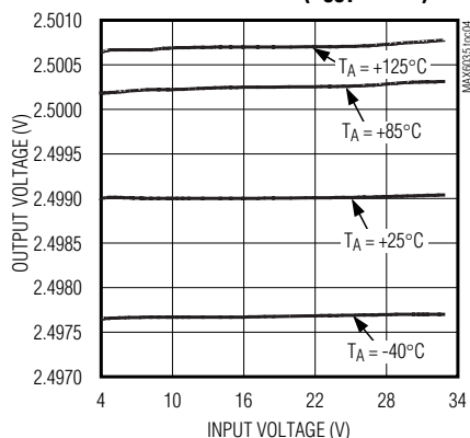
MAX6035 LINE REGULATION ( V_{OUT} = 2.5V )
