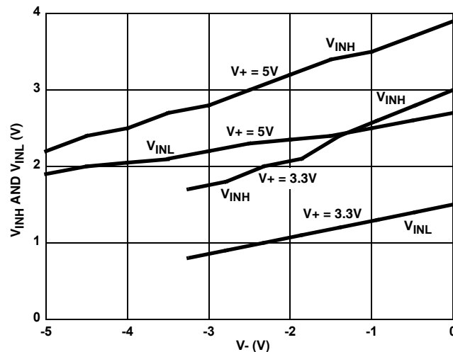
FIGURE 14. DIGITAL SWITCHING POINT vs NEGATIVE SUPPLY VOLTAGE
