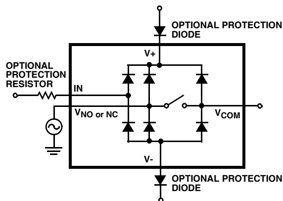
FIGURE 6. OVERVOLTAGE PROTECTION
