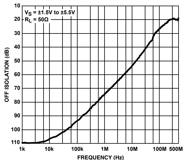
FIGURE 16. OFF ISOLATION
