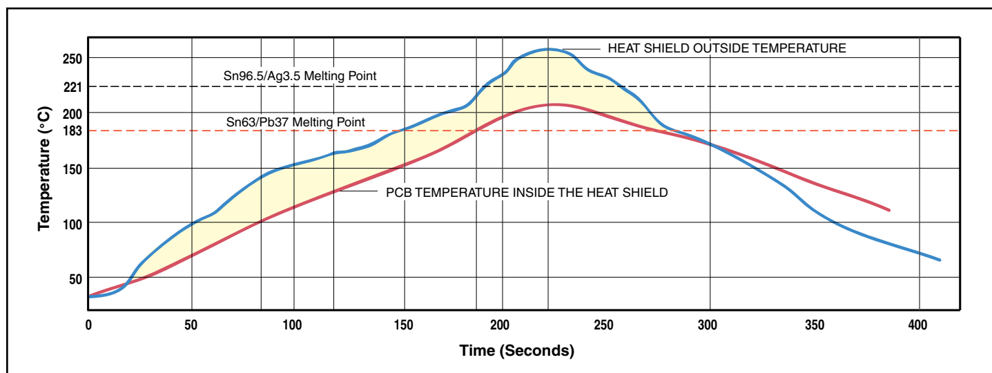
Figure 6. Reflow Solder Profile
