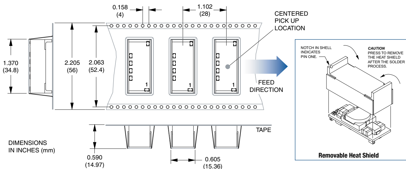
Figure 7. Tape Dimensions
