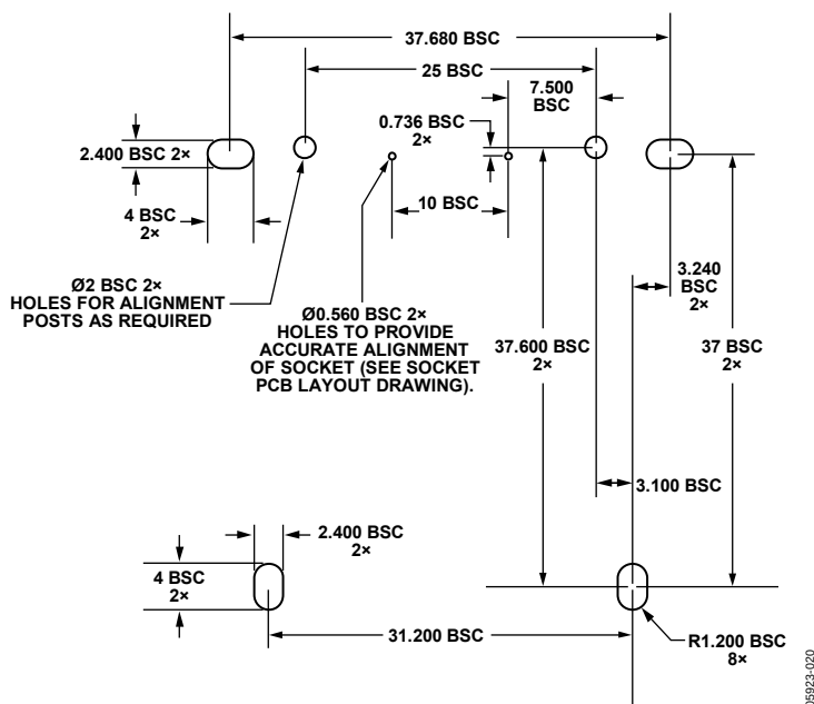
Figure 19. Printed Circuit Board Mounting Hole Pattern
