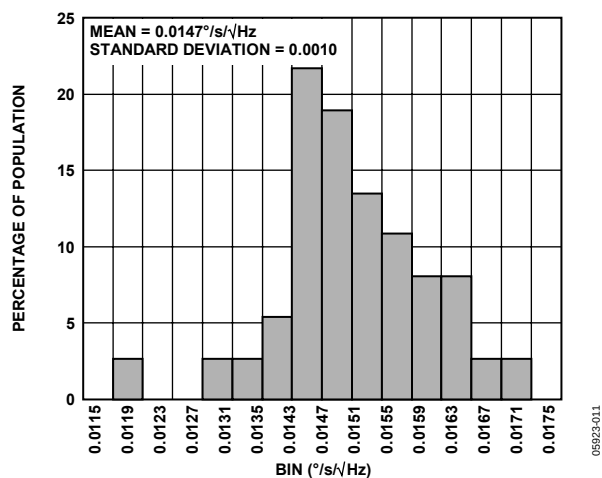
Figure 11. Noise Histogram
