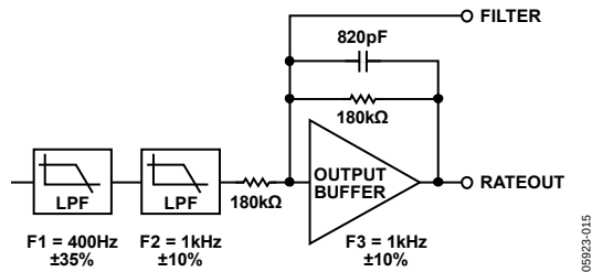
Figure 14. Simplified Filtering Network
