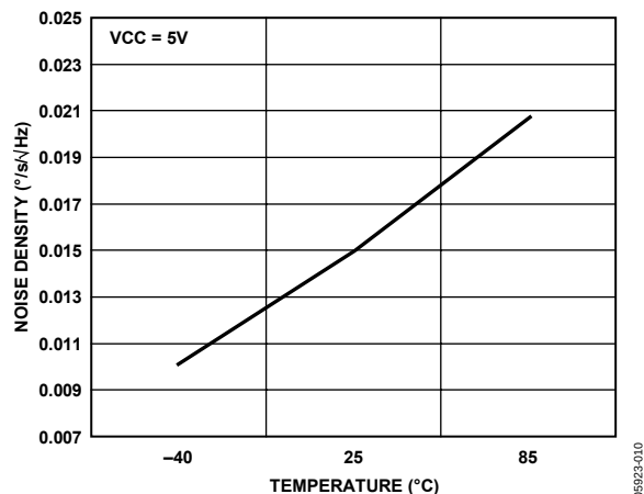
Figure 10. Noise Density vs. Temperature, VCC = 5 V
