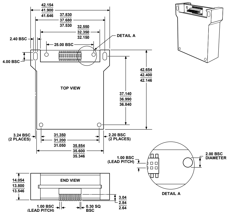
Figure 20. ADIS16120 PCB Module with Connector Interface (ML-24-1)
