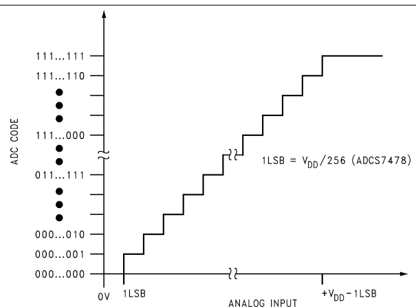
Figure 34. ADCS7478 Ideal Transfer Characteristic
