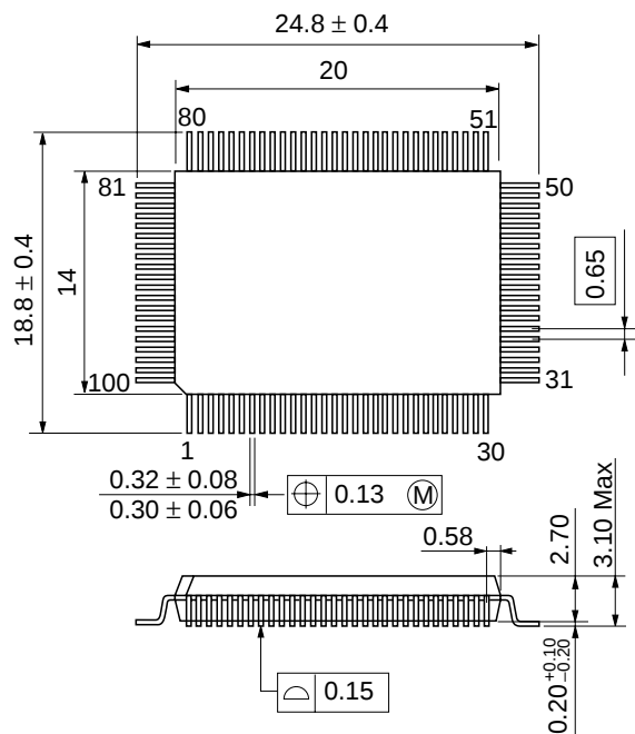
Figure F.2 FP-100A Package Dimensions
