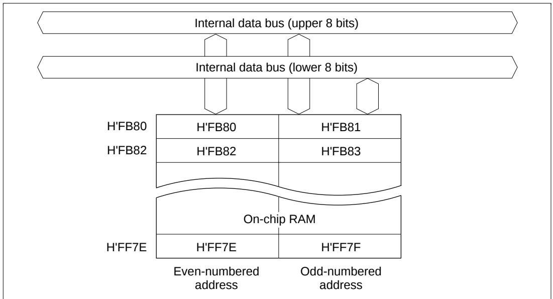
Figure 7.1 RAM Block Diagram (H8/3834)
