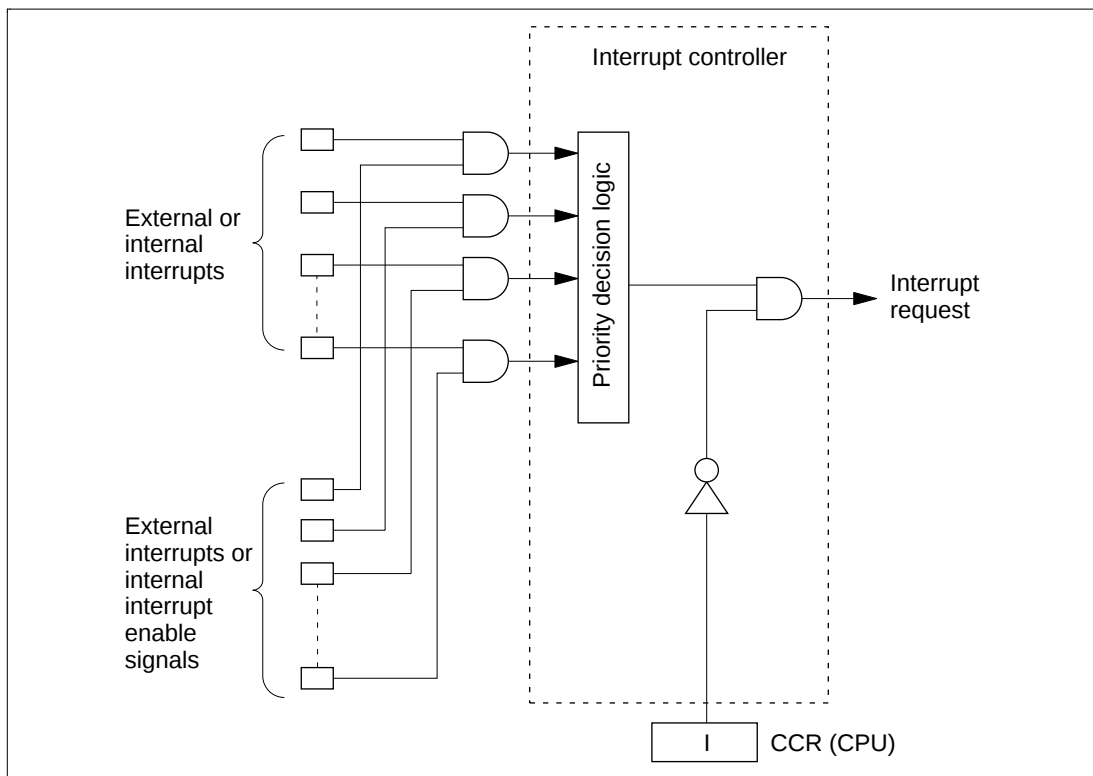
Figure 3.3 Block Diagram of Interrupt Controller
