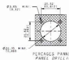
PERCAGES PANNEAU PANEL DRILLING
