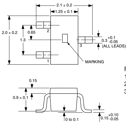
PACKAGE OUTLINE 30
