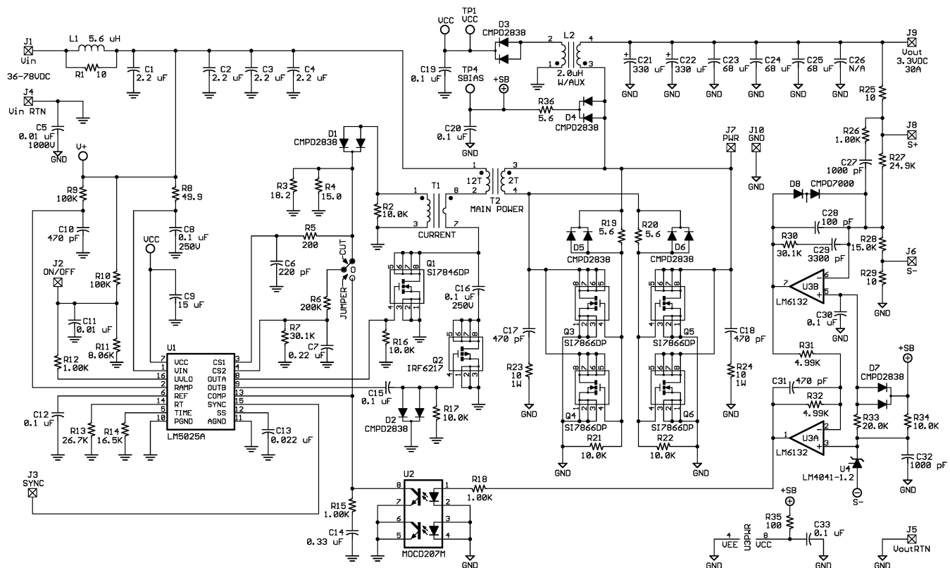
Figure 16. Application Circuit
