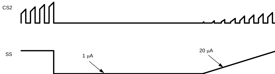
Figure 15. Current Limit
