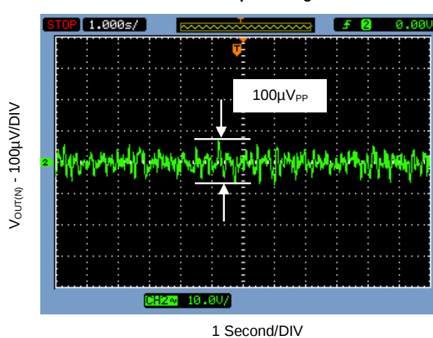
0.1Hz to 10Hz Output Voltage Noise
