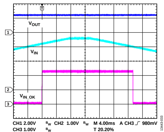
Figure 33. VINOK Function at VINOK Threshold = 3.0 V
