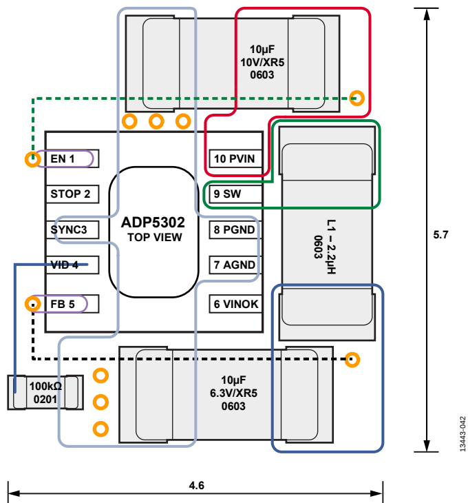
Figure 42. Typical PCB Layout for the ADP5302
