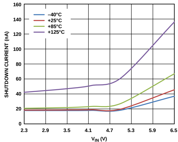
Figure 12. Shutdown Current vs. V_{IN} EN = Low
