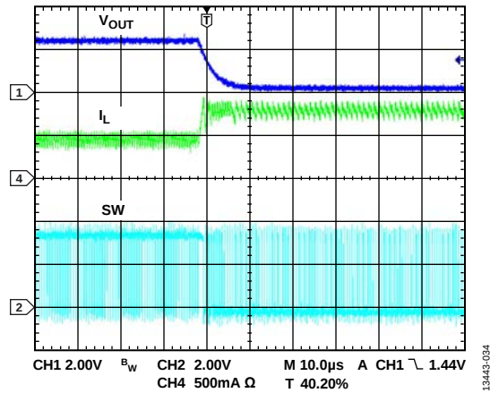
Figure 34. Output Short
