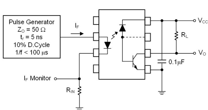
Figure 9 Transient Immunity Test Circuit &
