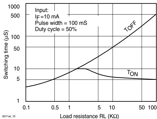
Figure 10. Typical Switching Times vs. Load Resistance
