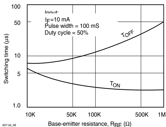
Figure 9. Typical Switching Characteristics vs. Base Resistance (Saturated Operation)
