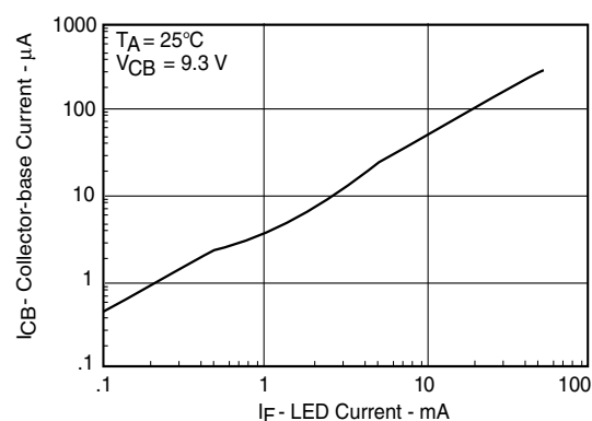
Figure 6. Collector-Base Photocurrent vs. LED Current
