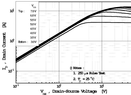
Fig 1. Output Characteristics
