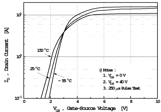
Fig 2. Transfer Characteristics
