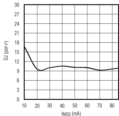
DETERMINISTIC JITTER vs. MODULATION AMPLITUDE
