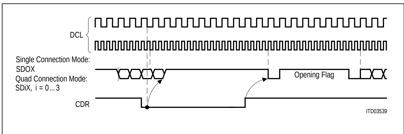
Figure 12 Transmission Control in the Slave Mode (example)
