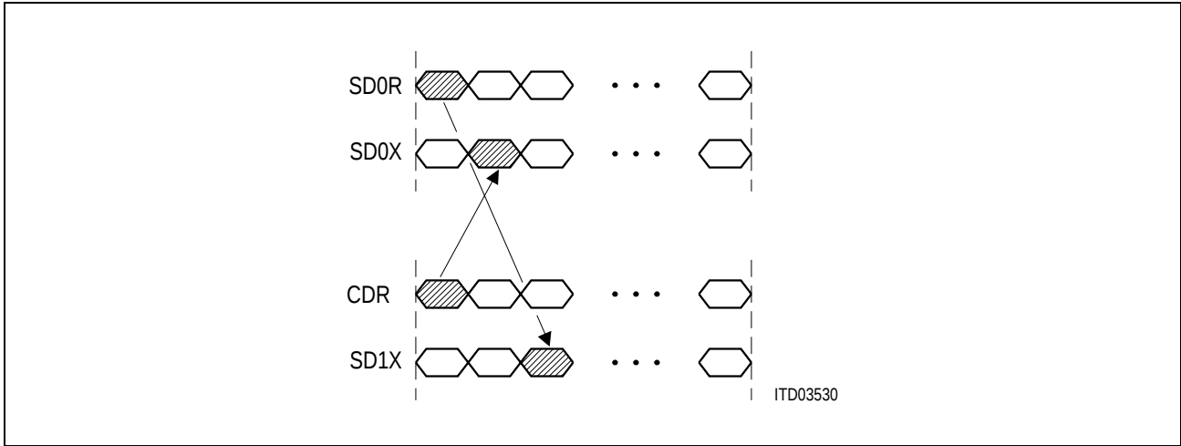
Figure 16a Bit Delay from SD0R/CDR to SD1X/SD0X
