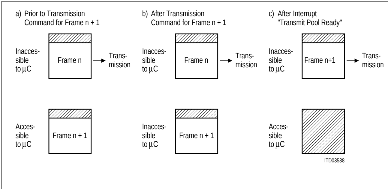
Figure 11 Transmit FIFO
