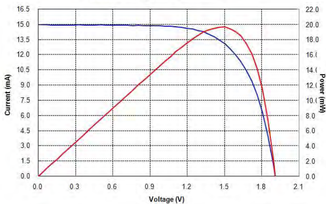
Current-Voltage Characteristics
