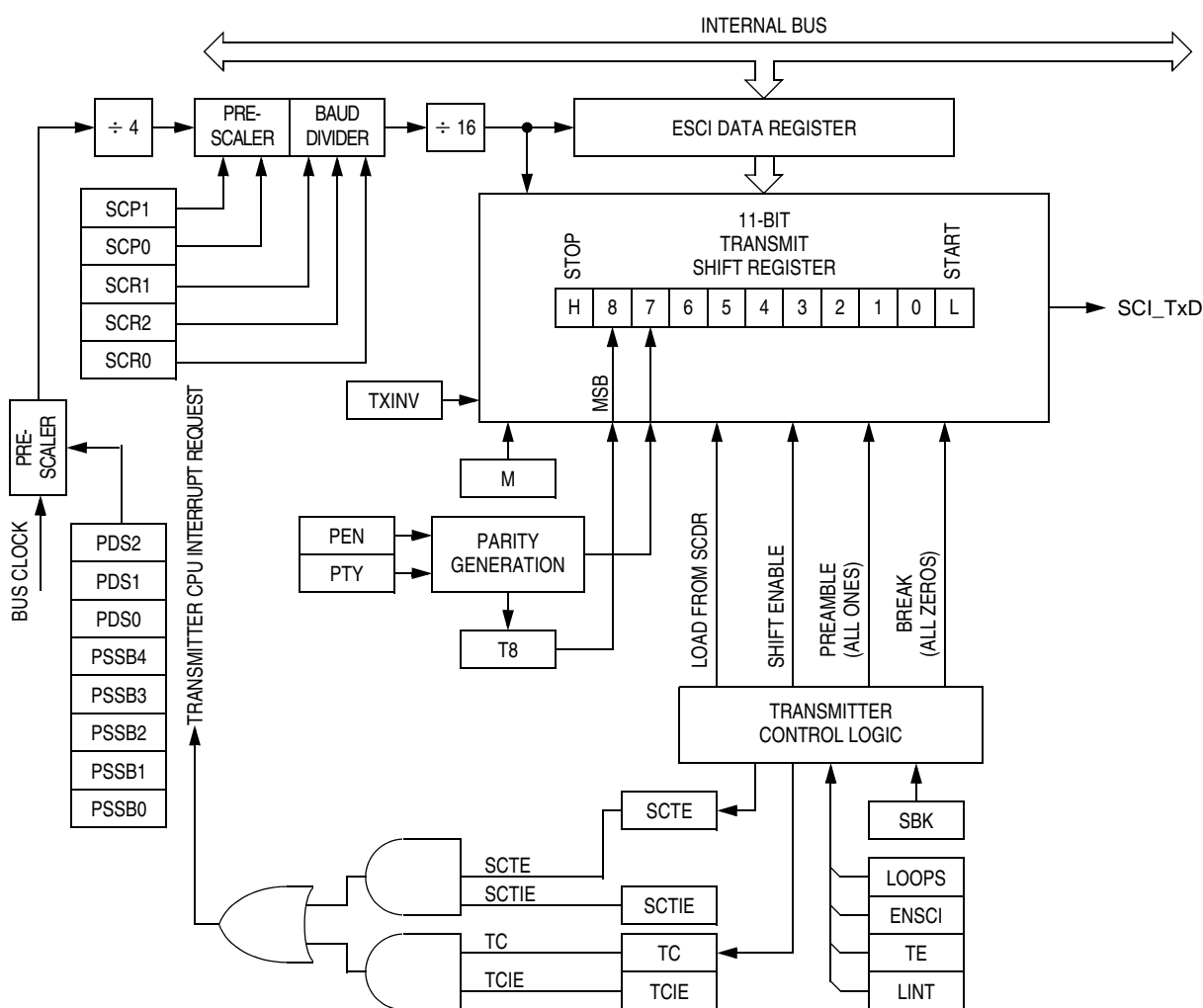
Figure 19-4. ESCI Transmitter
