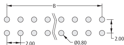
Recommended PC Board Pattern
