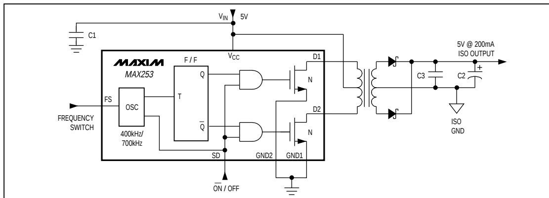
Figure 2. Block Diagram
