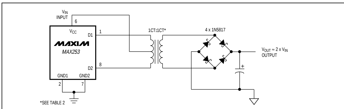
Figure 9c. Full-Wave Rectifier—Unipolar
