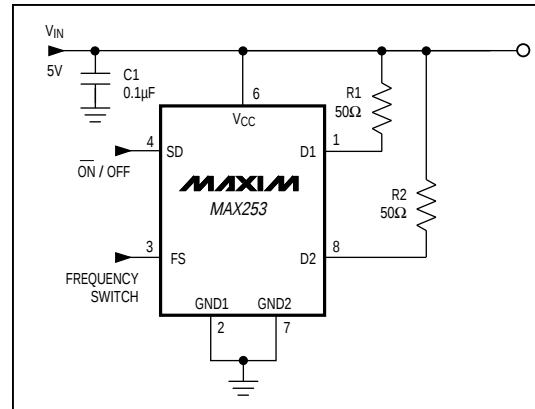
Figure 1. Test Circuit
