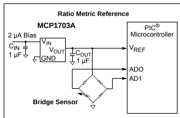
FIGURE 6-2: Using the MCP1703A as a Voltage Reference.
