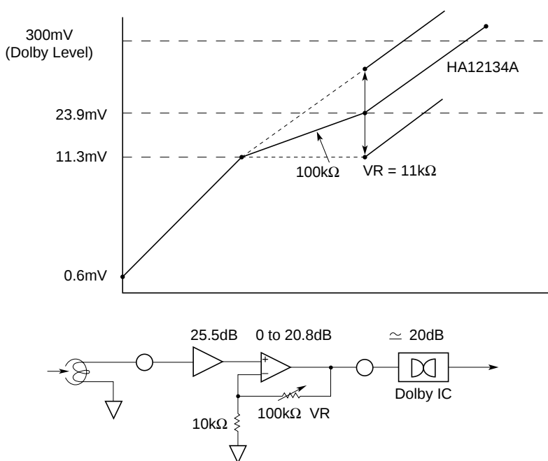
Figure 3 PB Level Diagram (Normal Speed, Normal Tape, 1kHz)
