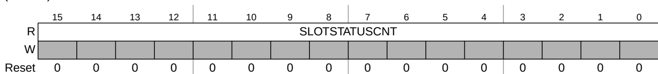
Figure 13-48. Slow Status Counter Registers (SSCR0–SSCR3)
