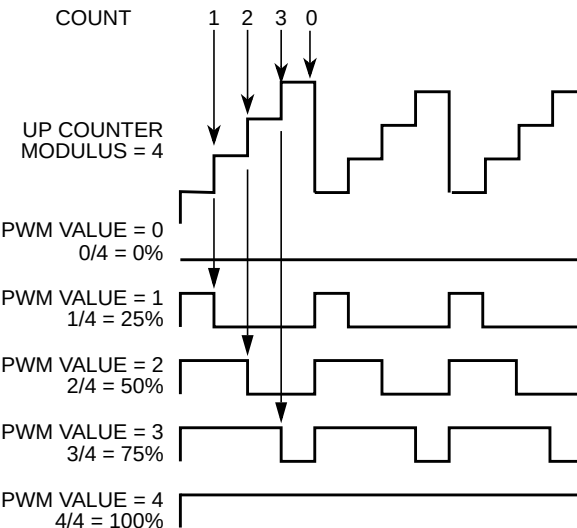
Figure 20-46. Edge-Aligned PWM Pulse Width
