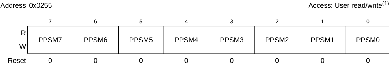
Figure 19-40. Port M Polarity Select Register (PPSM)
