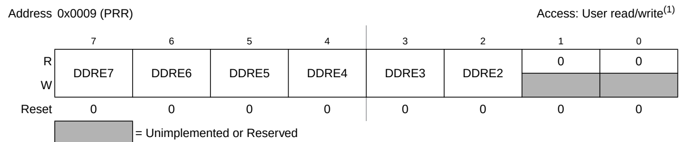
Figure 19-10. Port E Data Direction Register (DDRE)
