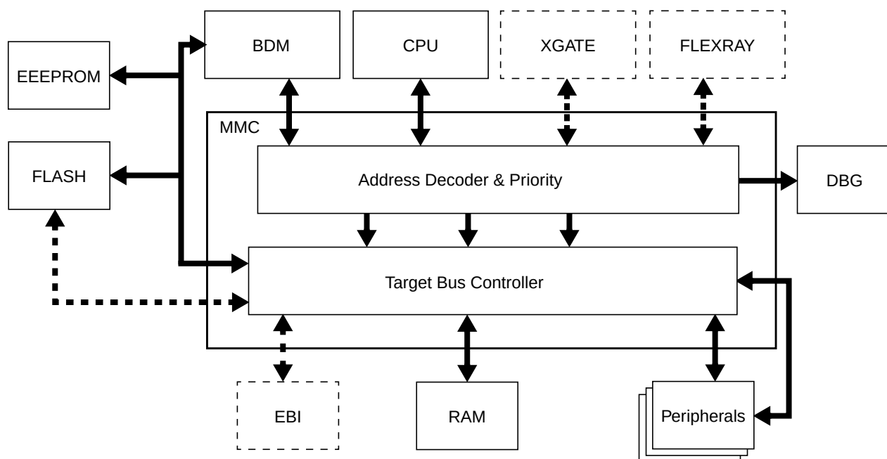
Figure 11-1. MMC Block Diagram
