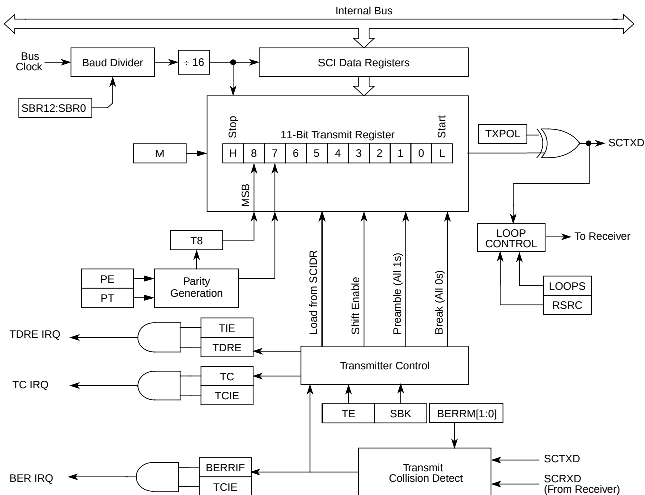
Figure 23-16. Transmitter Block Diagram
