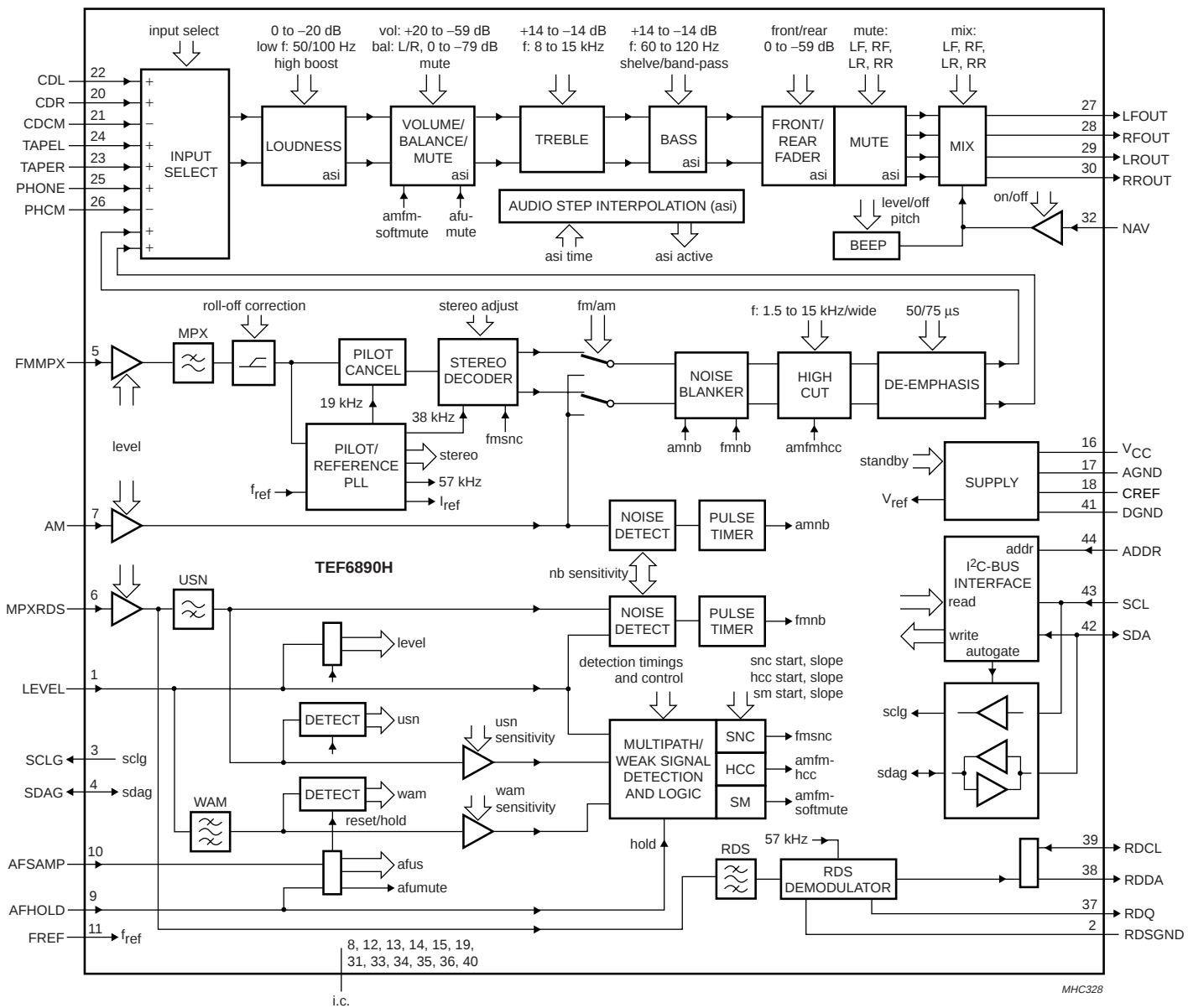
Fig.1 Block diagram.
