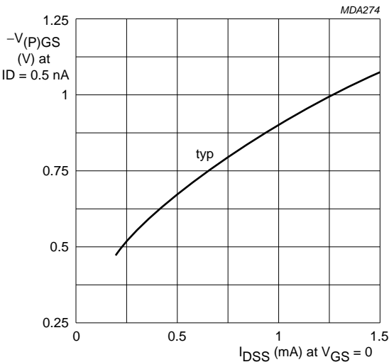
Fig.5 Correlation between -V_{(P)GS} and I_{DSS} . V_{DS} = 10\text{ V} ; T_j = 25\text{ °C} .
