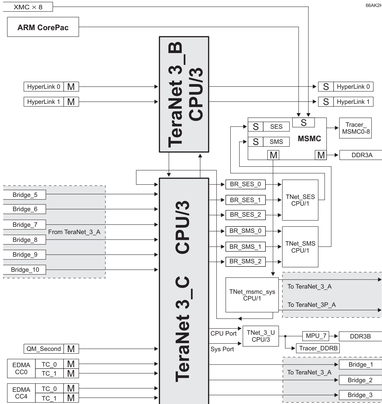
Figure 9-3. TeraNet 3_C
