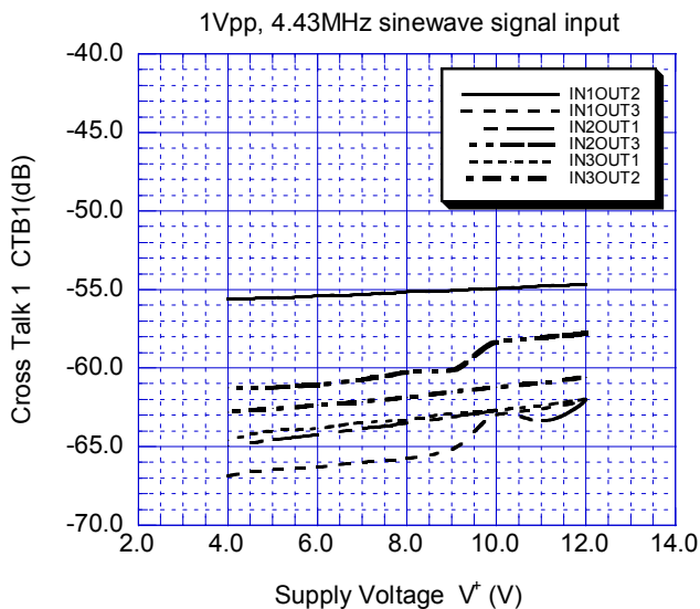
Cross Talk 1 vs. Supply Voltage
