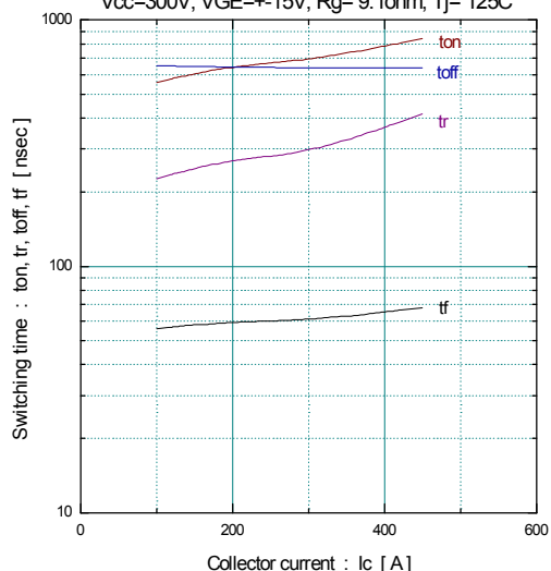
[ Inverter ] Switching time vs. Collector current (typ.) V_{cc}=300V , V_{GE}=\pm 15V , R_g=9.1\Omega , T_j=125^\circ C
