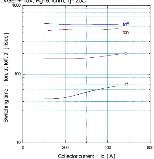
[ Inverter ] Switching time vs. Collector current (typ.) V_{cc}=300V , V_{GE}=\pm 15V , R_g=9.1\Omega , T_j=25^\circ C
