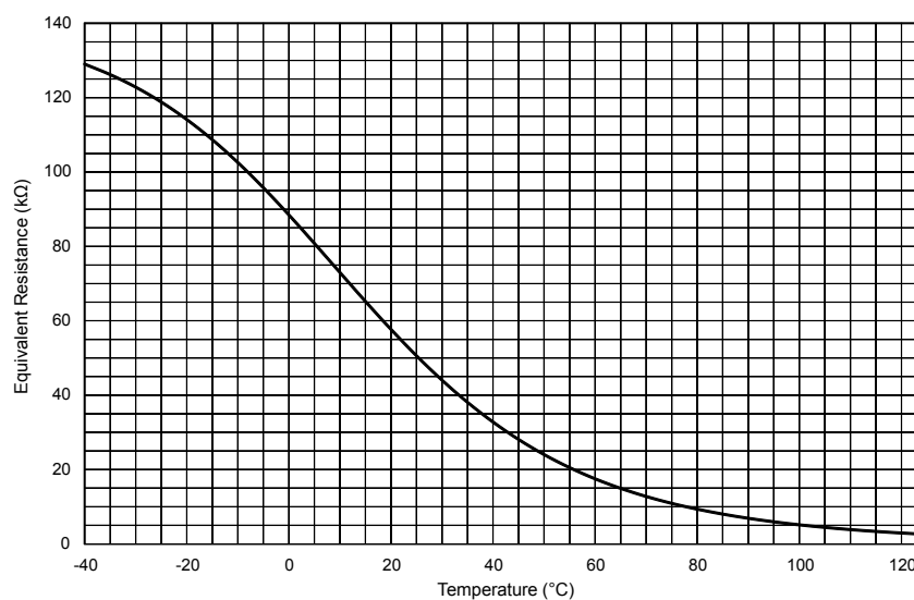
Figure 6. Equivalent resistance ( \text{NTC} // \text{R}_{\text{PD\_SD}} )
