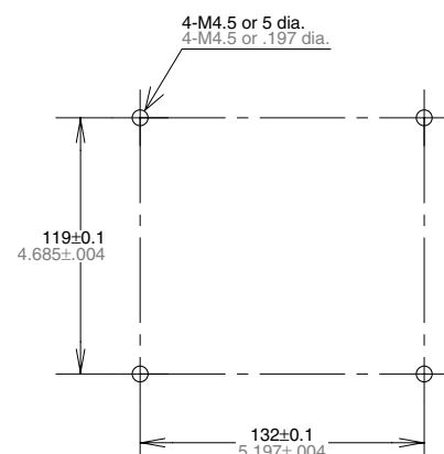
Mounting dimensions
