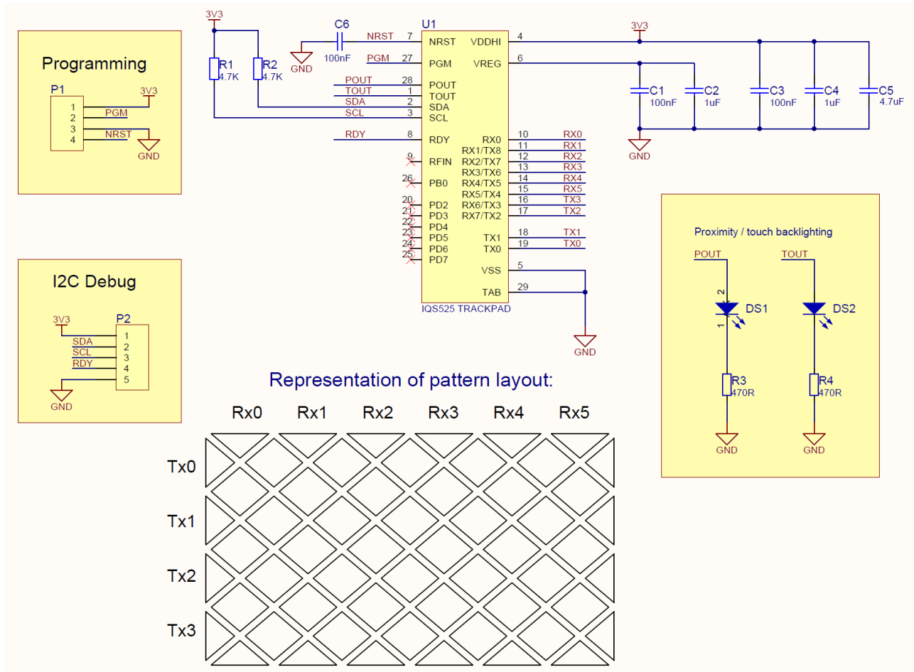
Figure 6.5 IQS525 Application Circuit
