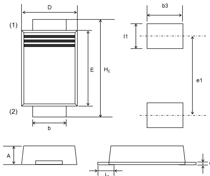
SOD-128, (PMDTM)
