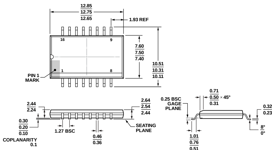
COMPLIANT TO JEDEC STANDARDS MS-013-AC Figure 26. 16-Lead Standard Small Outline Package, with Increased Creepage [SOIC_IC] Wide Body (RI-16-2) Dimensions shown in millimeters
