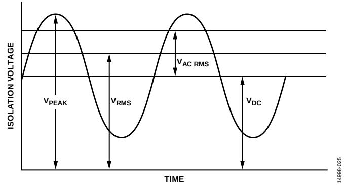
Figure 25. Critical Voltage Example
