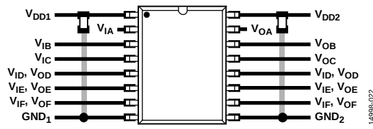
Figure 22. Recommended Printed Circuit Board Layout
