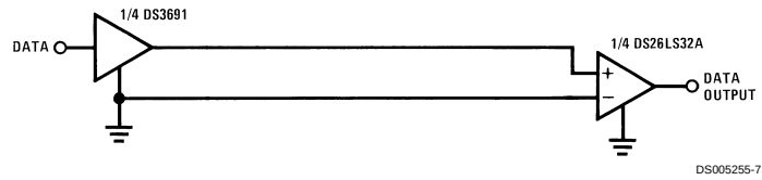
Single Wire with Driver Ground Reference—RS-423
