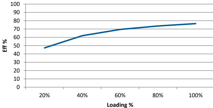
AM1PS-2405SZ Efficiency vs. Loading
