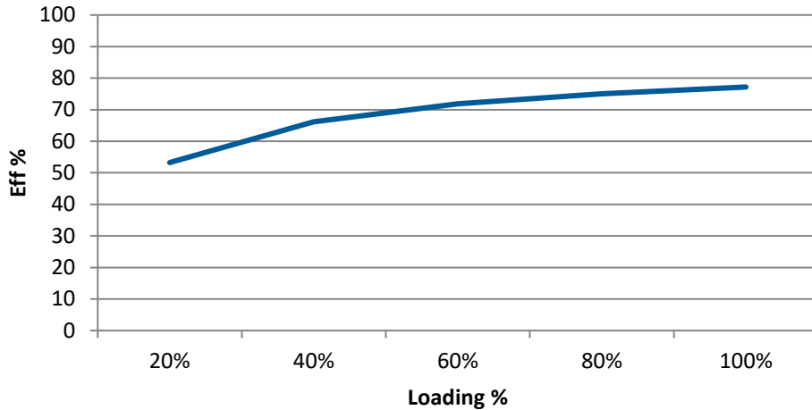
AM1PS-1205SZ Efficiency vs. Loading
