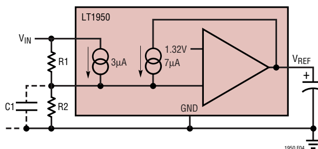
Figure 4. Undervoltage Lockout
