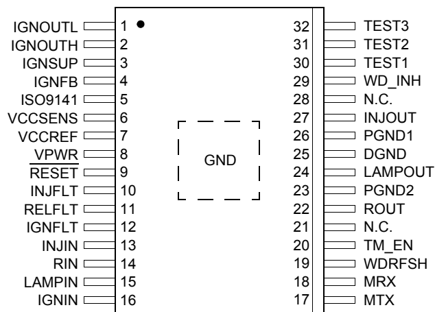
Figure 4. 33812 Pin Connections
