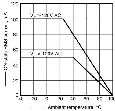
1-(5). ON-state RMS current vs. ambient temperature characteristics Allowable ambient temperature: -40^{\circ}\text{C} to +100^{\circ}\text{C} -40^{\circ}\text{F} to +212^{\circ}\text{F} Tested sample: APT1212(A), APT1222(A), APT1212W(A), APT1222W(A)
