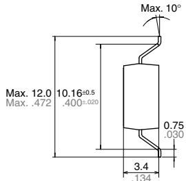
Surface mount terminal type
