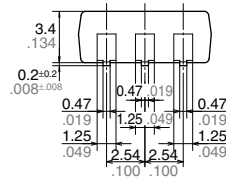
Recommended mounting pad (TOP VIEW)
