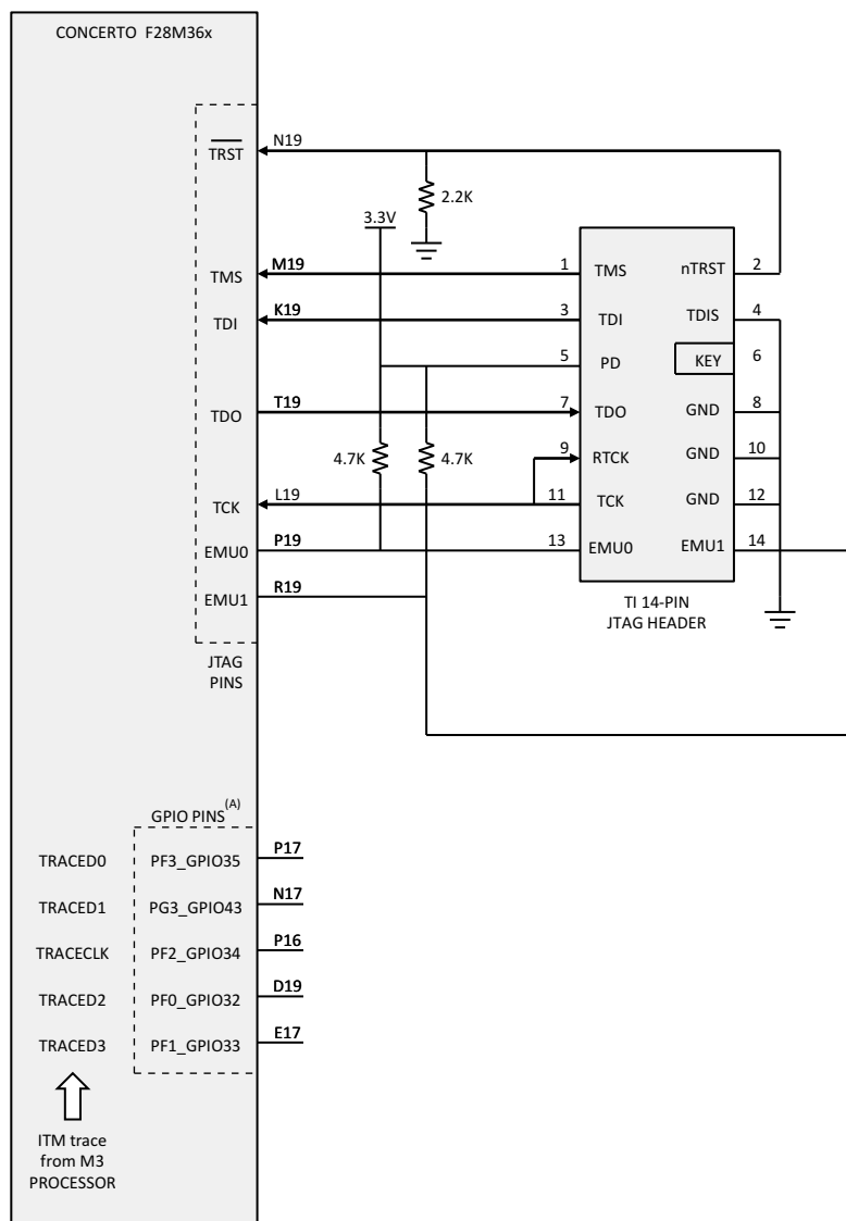
Figure 2-18. Connecting to TI 14-Pin JTAG Emulator Header
