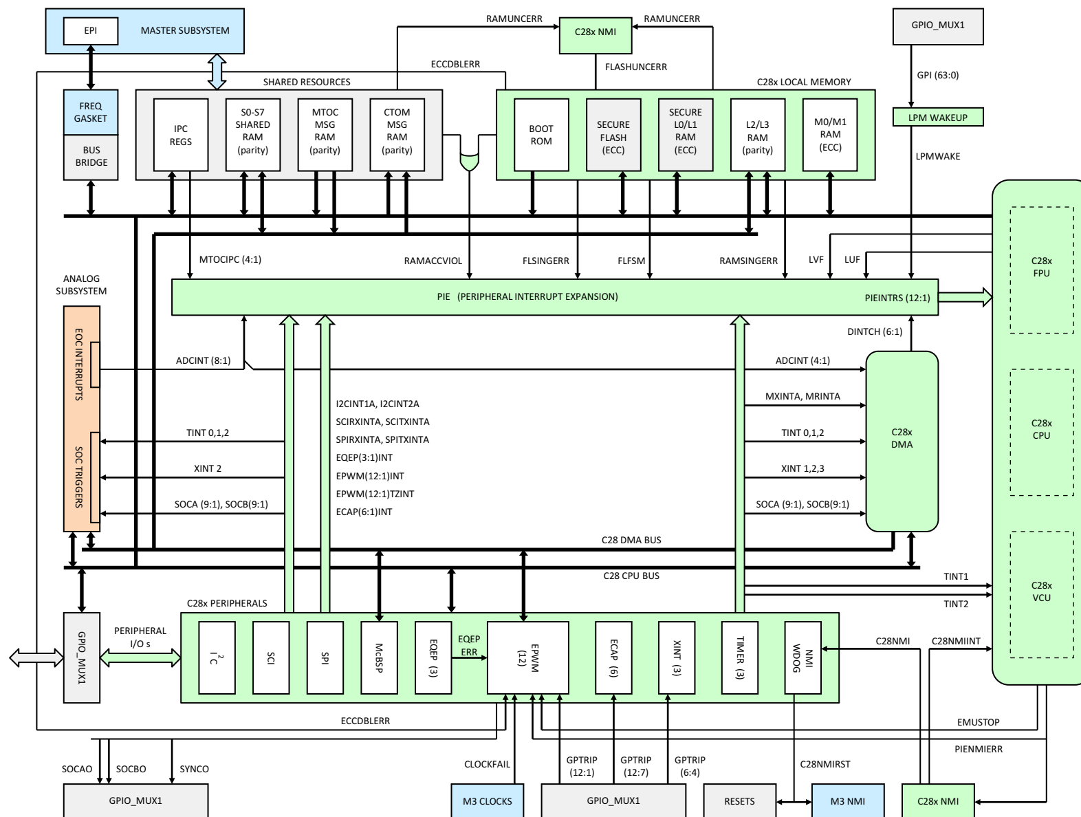
Figure 2-2. Control Subsystem
