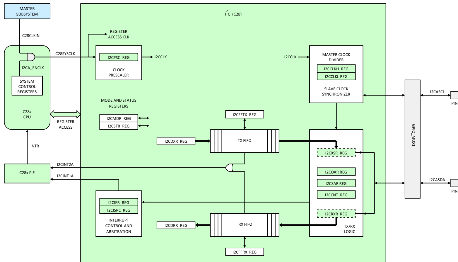
Figure 6-39. I 2 C (C28x)
