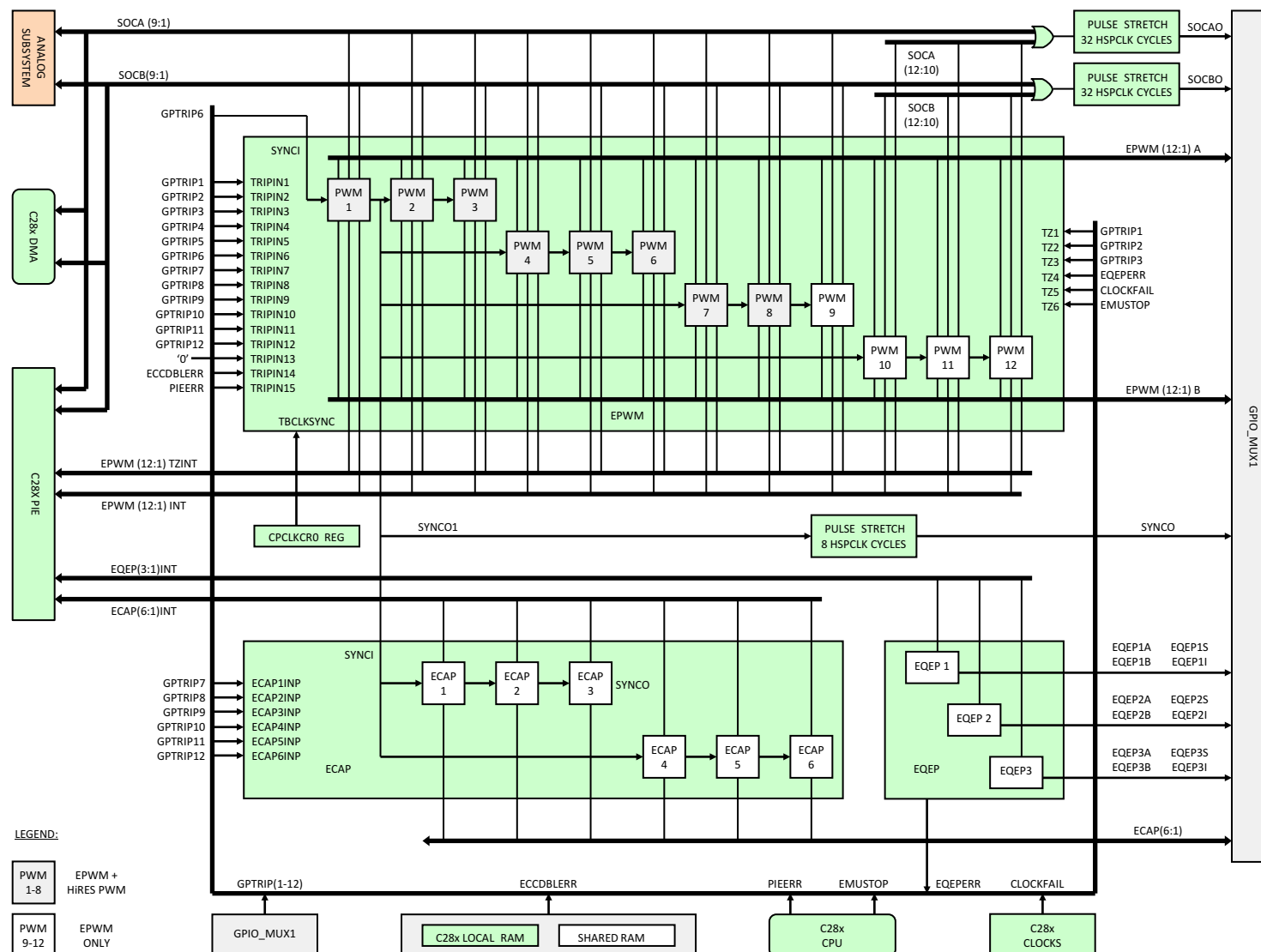
Figure 6-34. PWM, eCAP, eQEP
