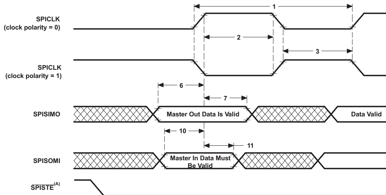
Figure 6-43. SPI Master Mode External Timing (Clock Phase = 1)
