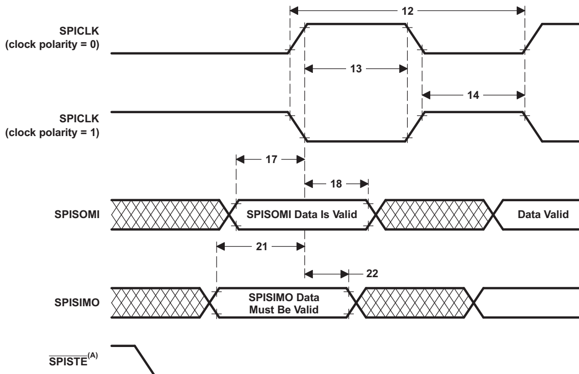
Figure 6-45. SPI Slave Mode External Timing (Clock Phase = 1)
