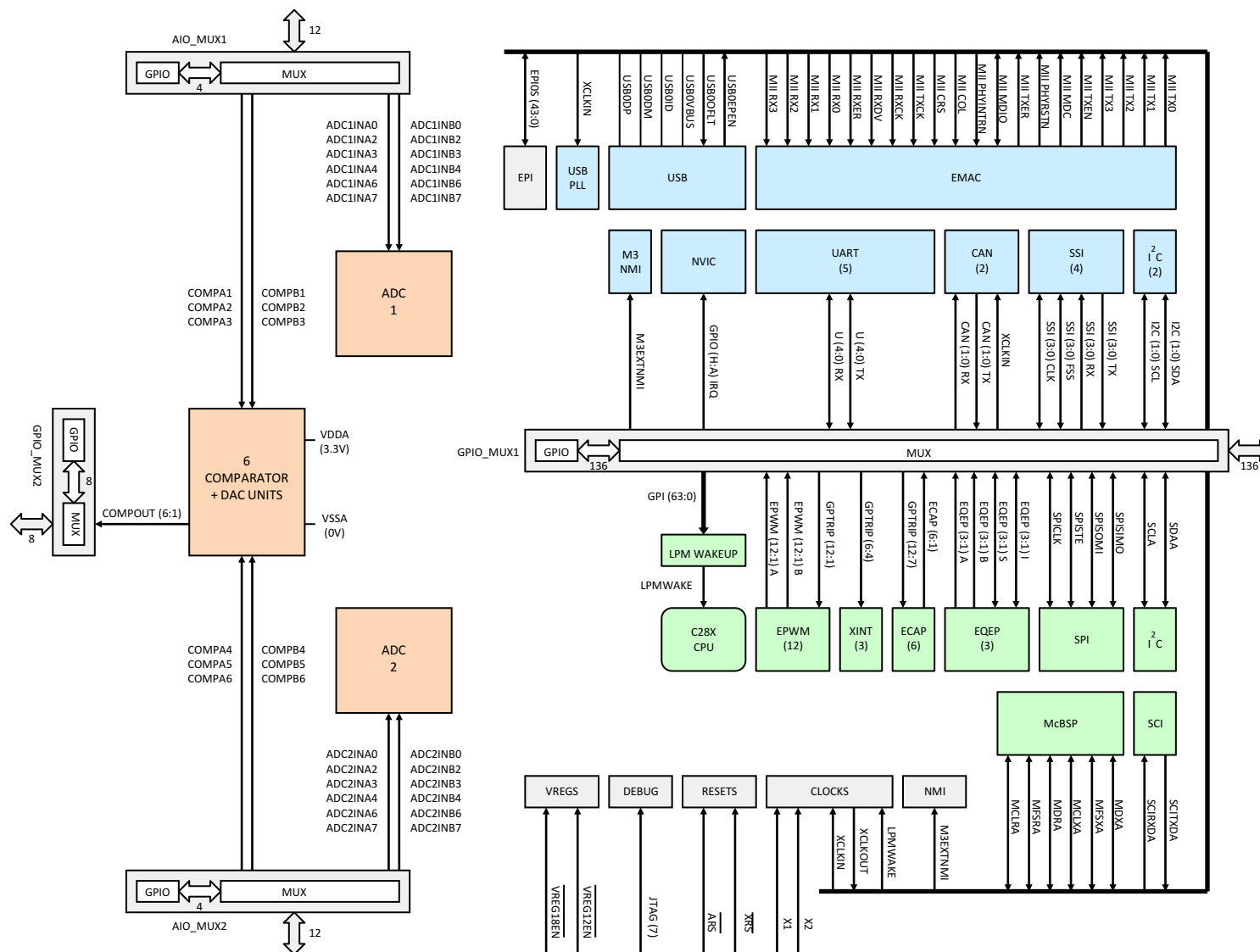
Figure 2-14. GPIOs and Other Pins
