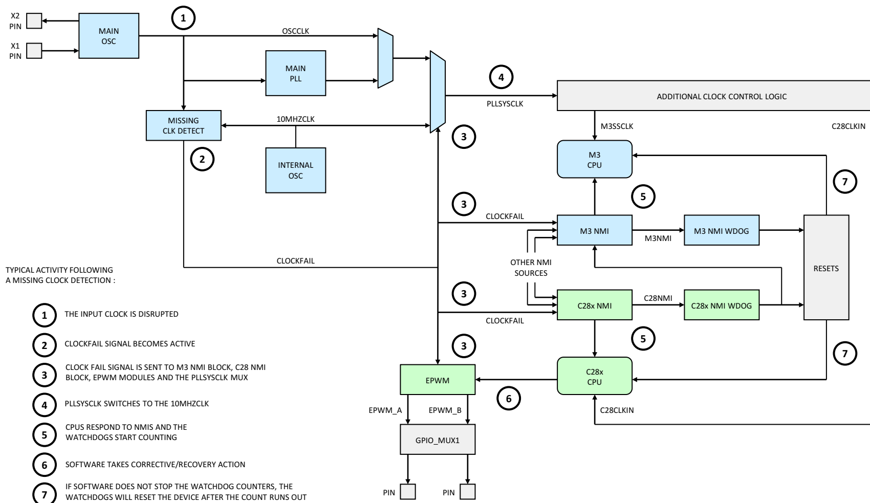
Figure 2-13. Missing Clock Detection
