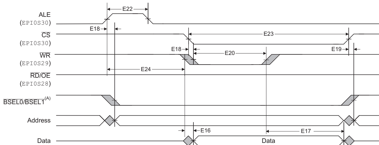
Figure 6-16. Host-Bus 8/16 Mode Write Timing
