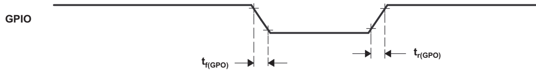
Figure 5-5. General-Purpose Output Timing
