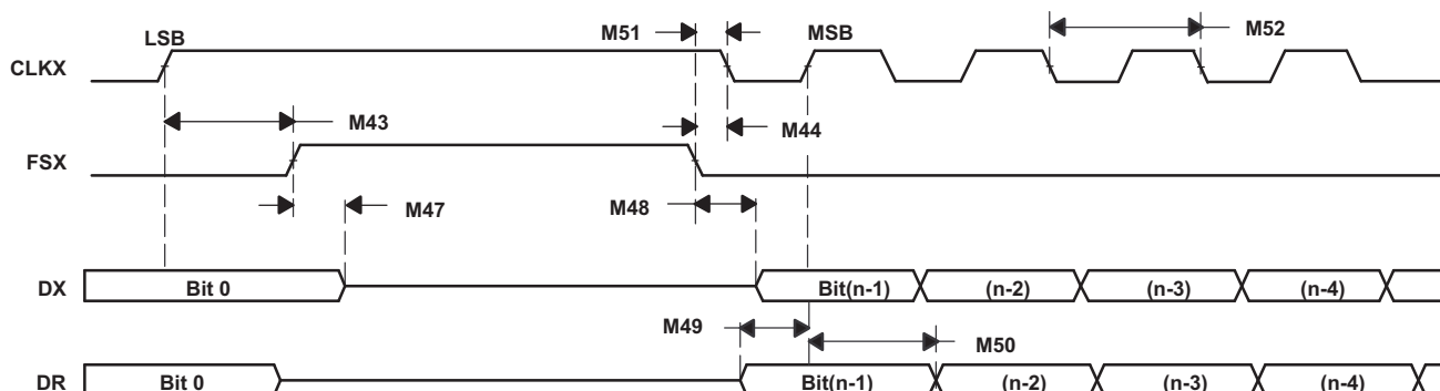
Figure 6-51. McBSP Timing as SPI Master or Slave: CLKSTP = 10b, CLKXP = 1
