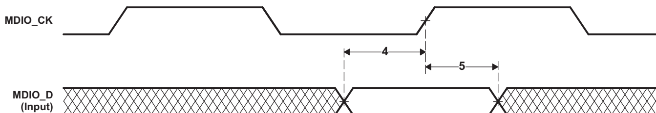
Figure 6-33. MII Serial Management Timing – MDIO as Input
