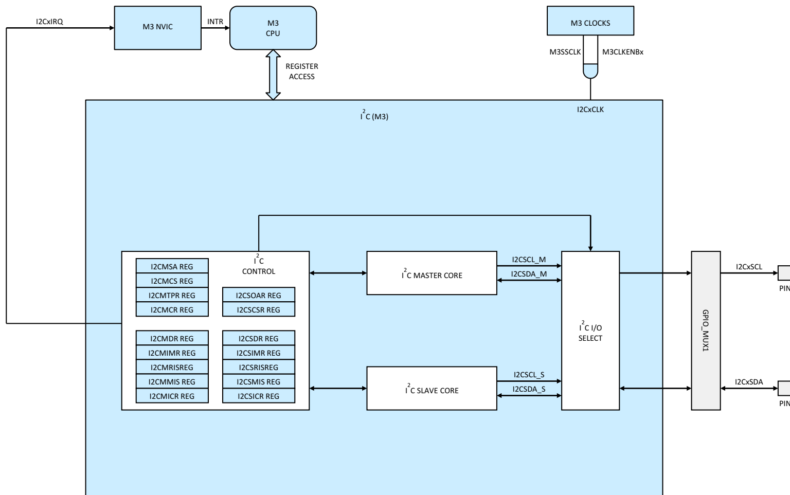
Figure 6-23. I 2 C (Cortex™-M3)
