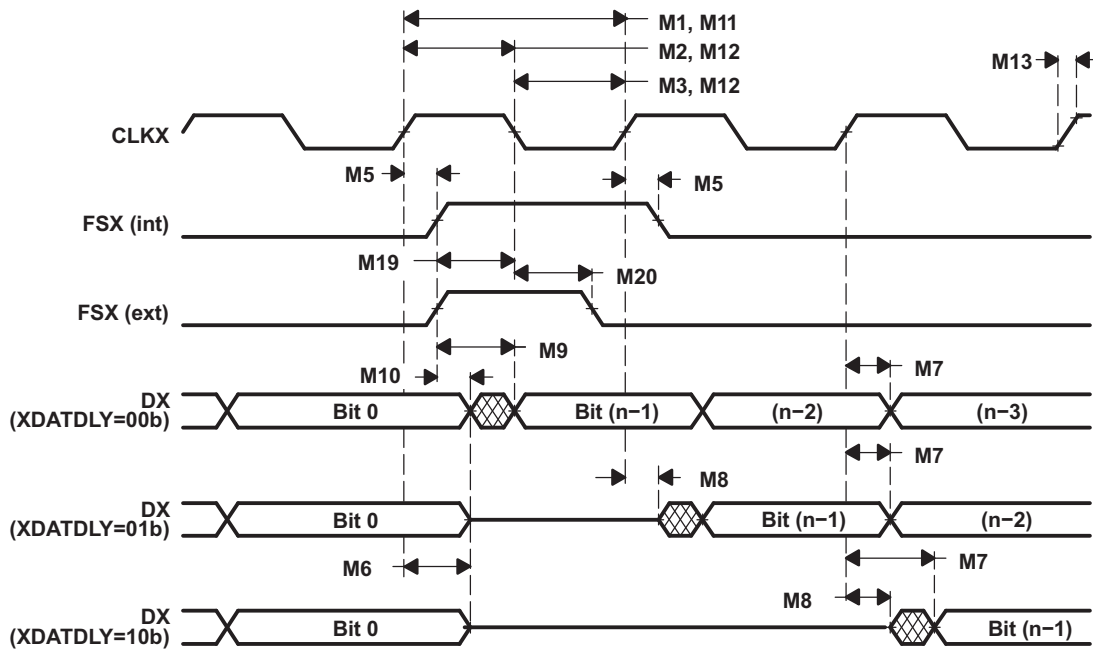
Figure 6-48. McBSP Transmit Timing
