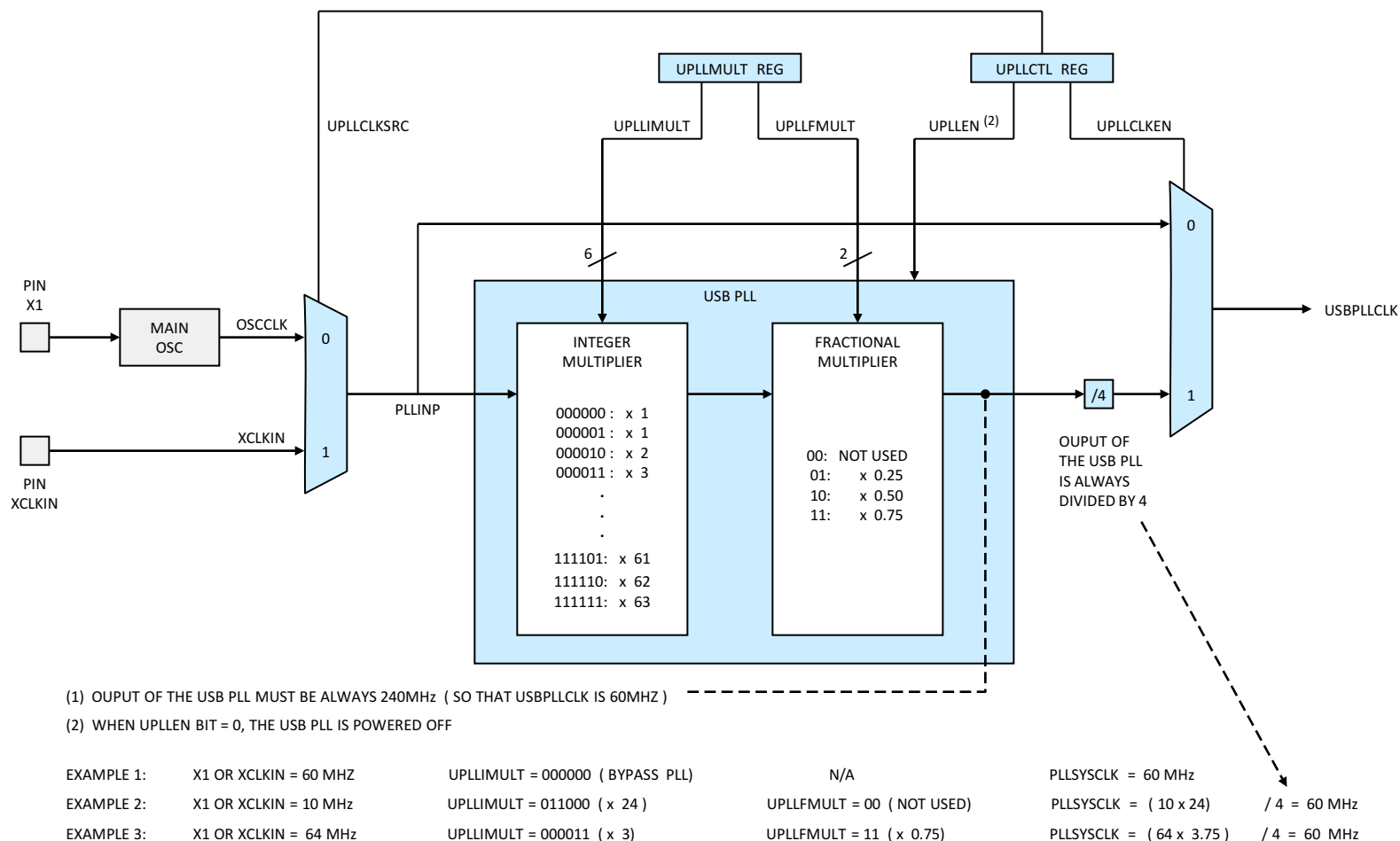
Figure 2-9. USB PLL
