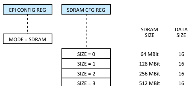
Figure 6-9. EPI SDRAM Mode
