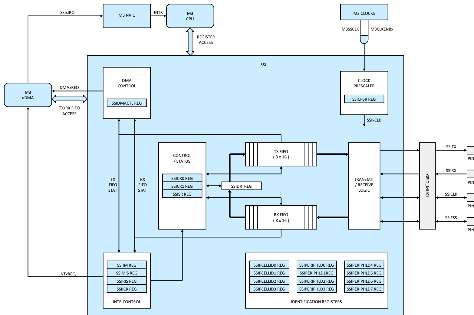
Figure 6-21. SSI
