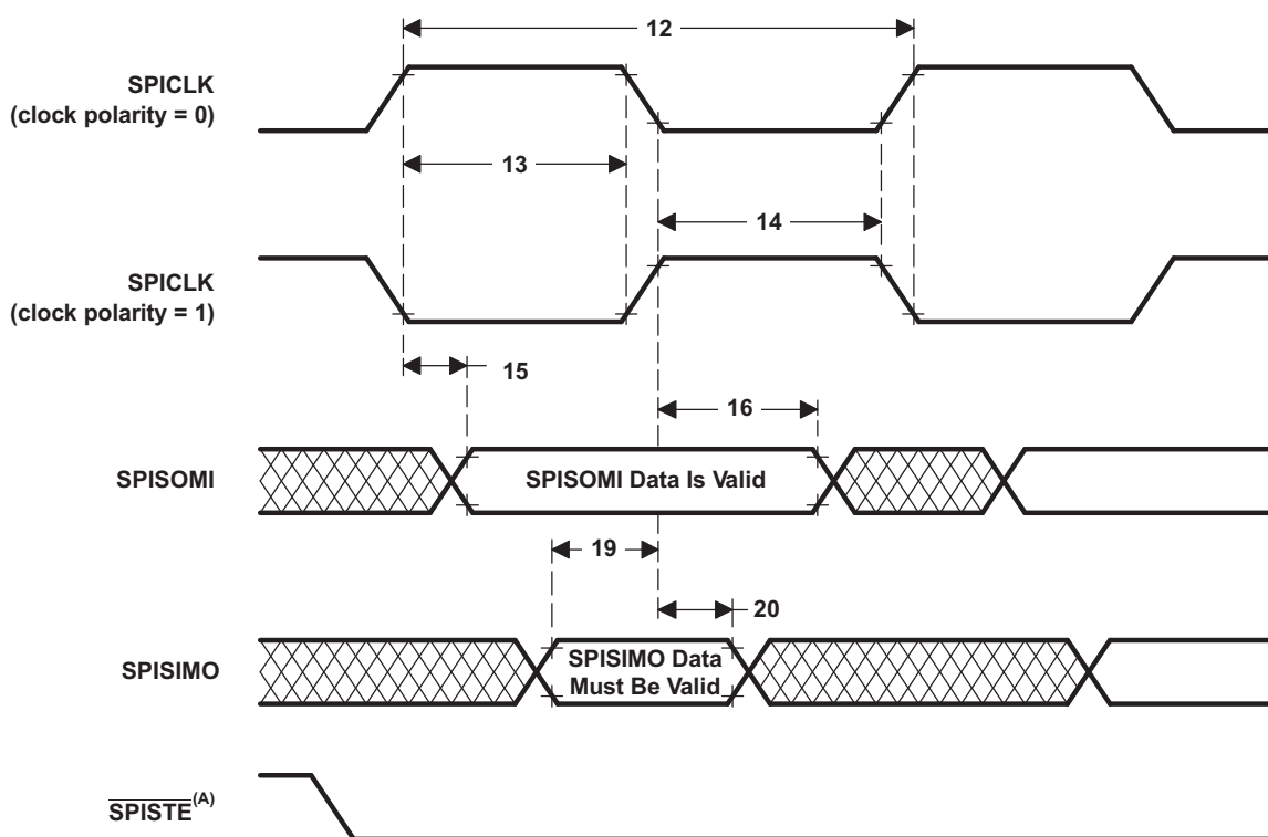
Figure 6-44. SPI Slave Mode External Timing (Clock Phase = 0)
