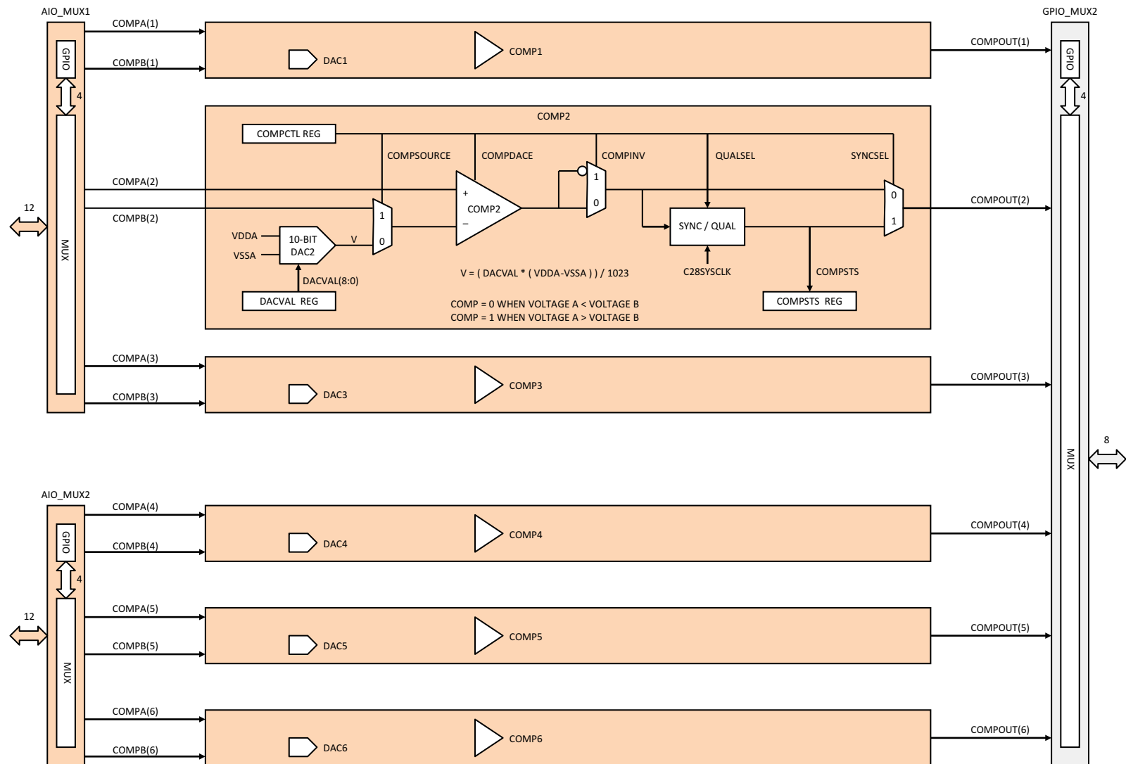
Figure 6-4. Comparator + DAC Units
