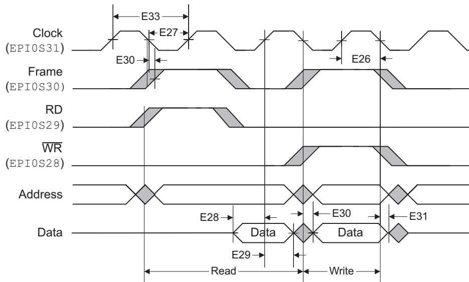
Figure 6-19. General-Purpose Mode Read and Write Timing
