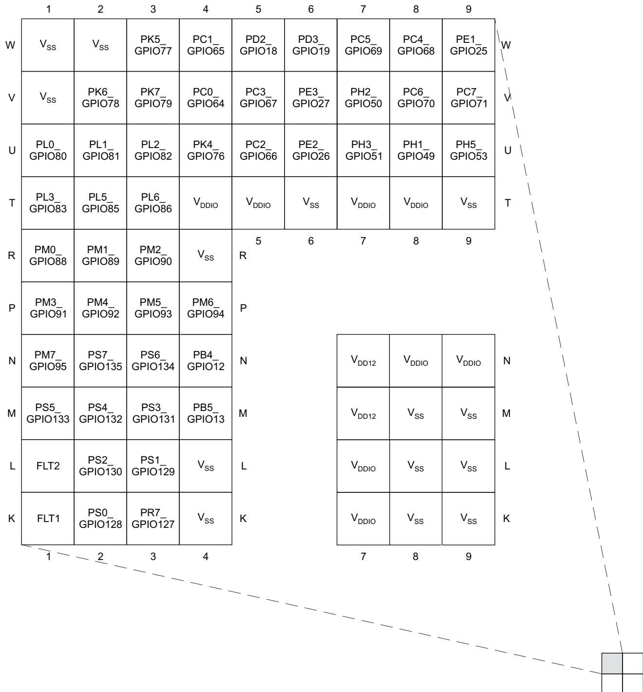
Figure 3-2. 289-Ball ZWT Pin Map [Quadrant A]
