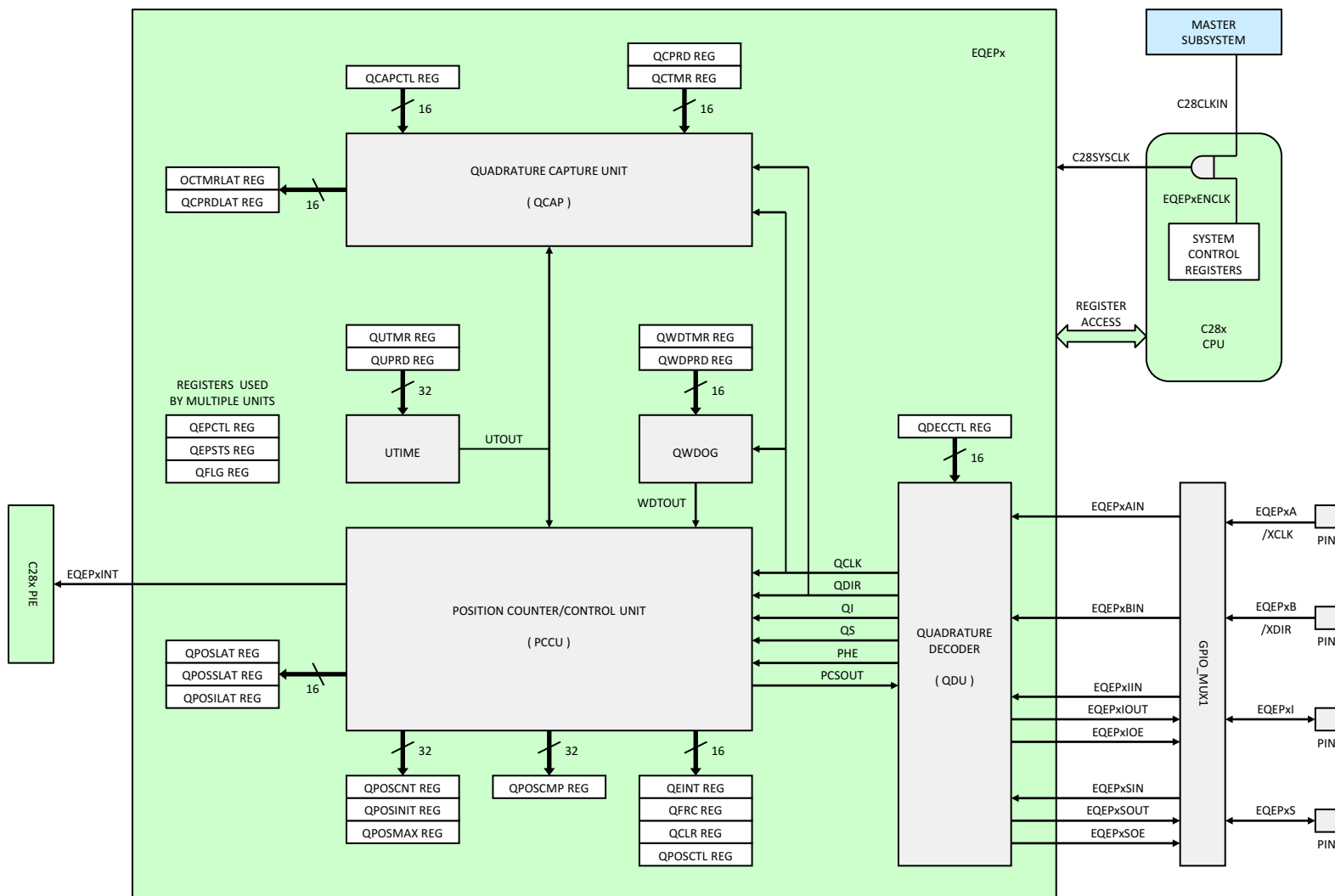
Figure 6-38. eQEP
