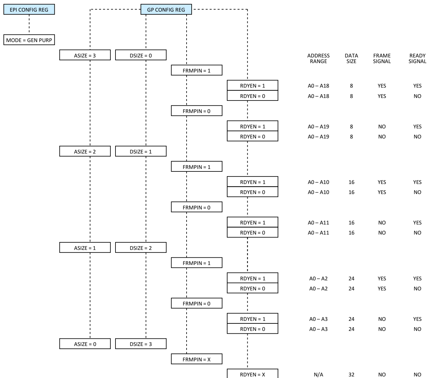
Figure 6-8. EPI General-Purpose Modes
