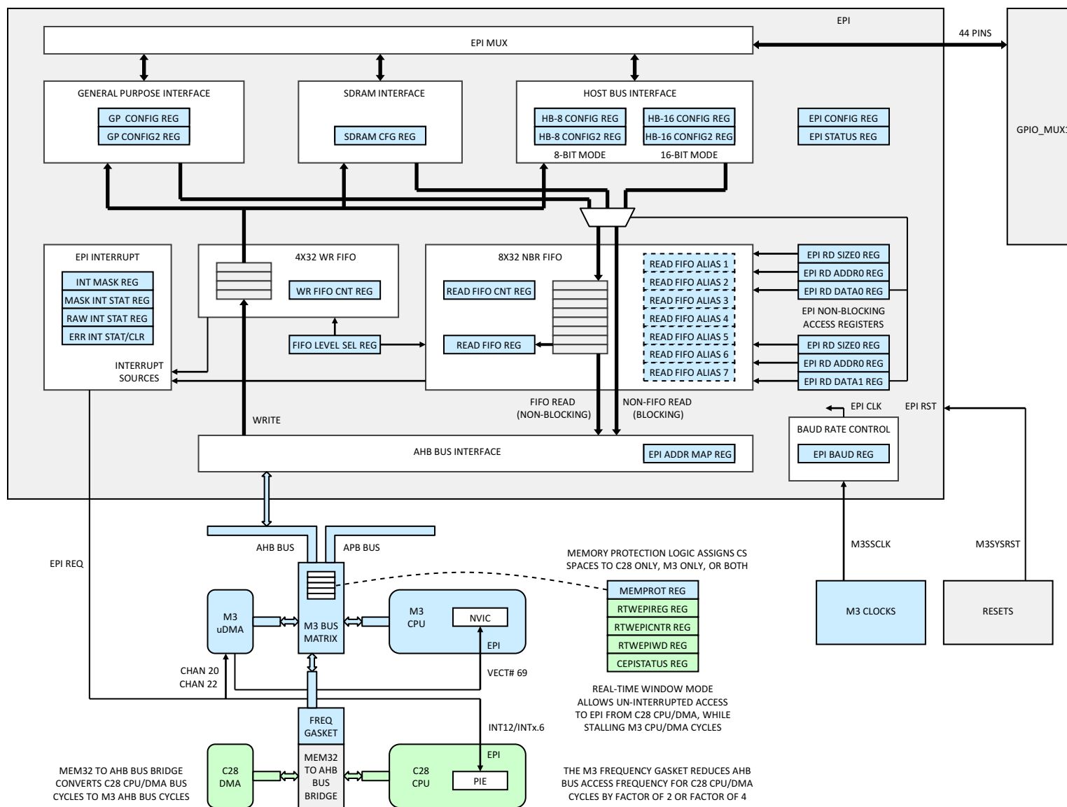
Figure 6-7. External Peripheral Interface (EPI)
