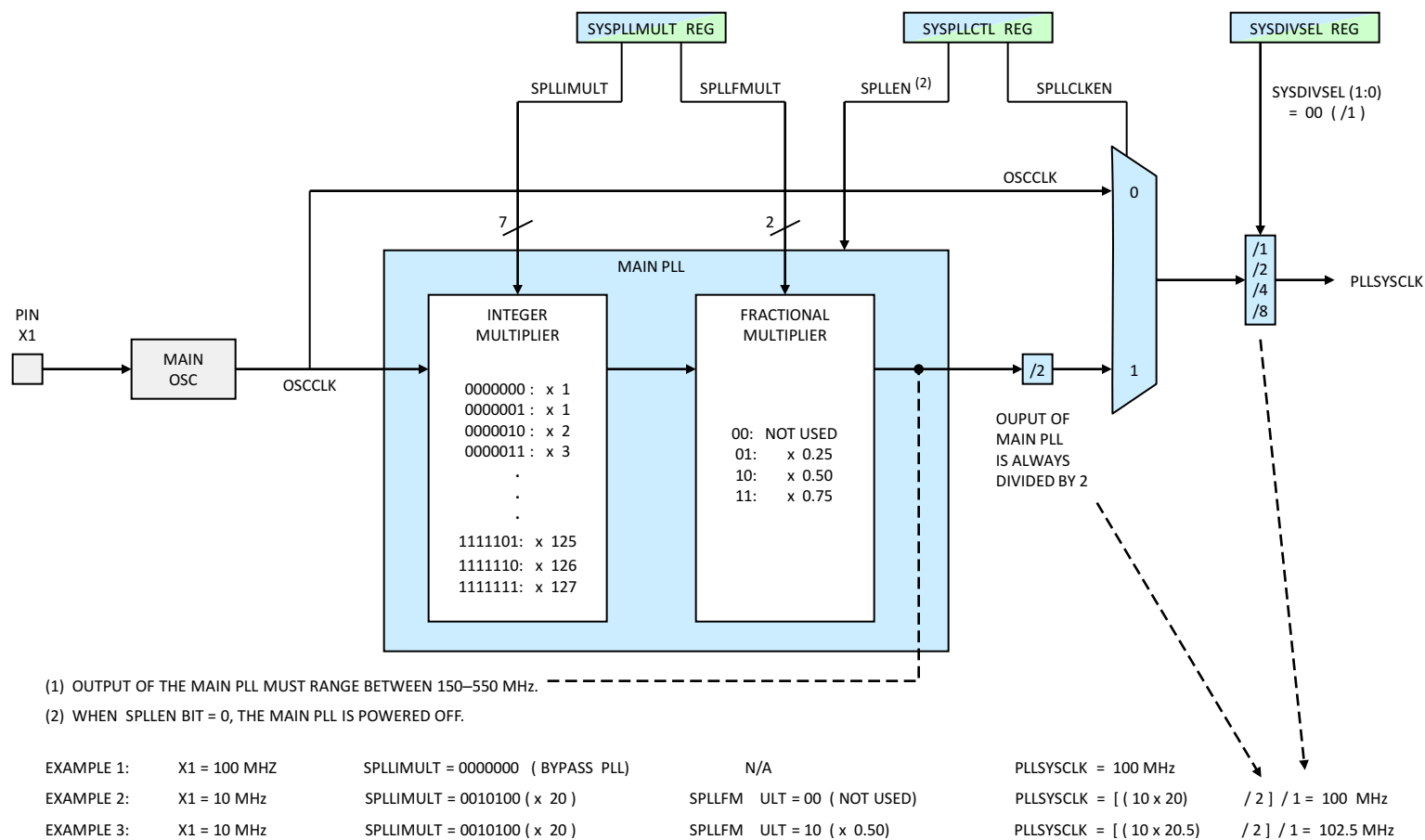
Figure 2-8. Main PLL
