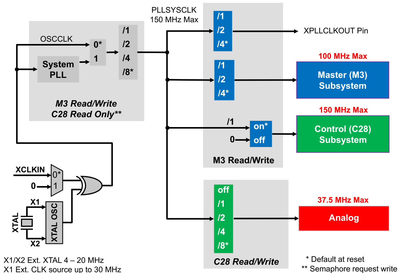
Figure 2-11. System Clock/PLL
