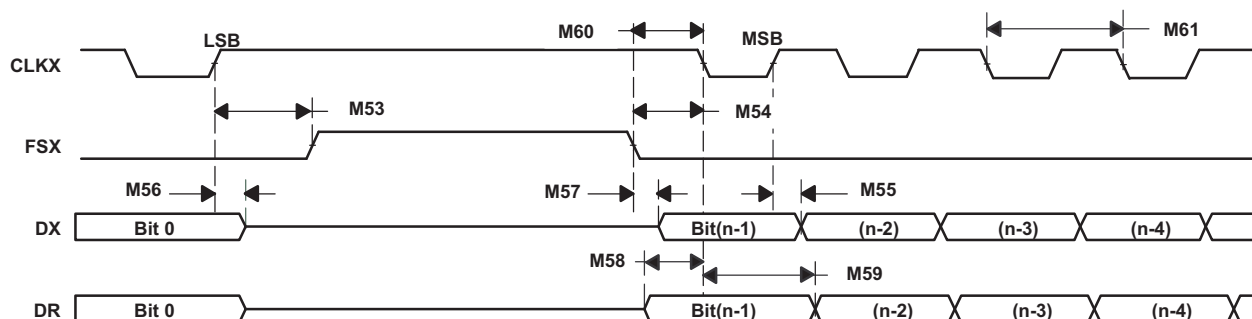
Figure 6-52. McBSP Timing as SPI Master or Slave: CLKSTP = 11b, CLKXP = 1
