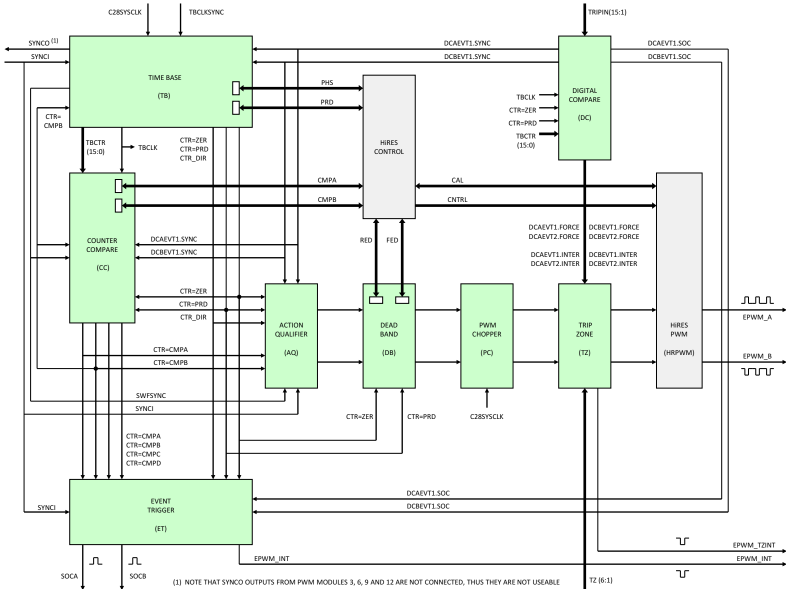
Figure 6-35. Internal Structure of PWM
