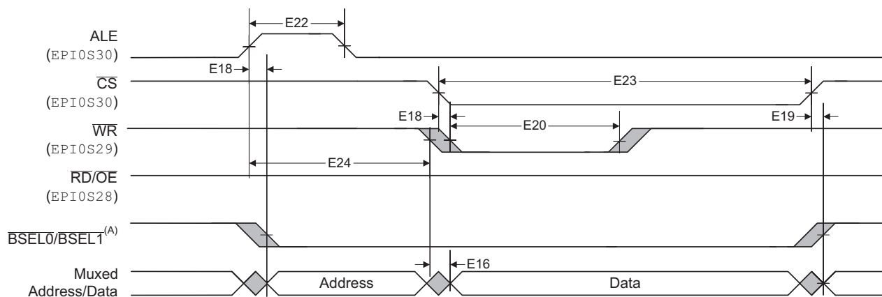
Figure 6-18. Host-Bus 8/16 Mode Muxed Write Timing
