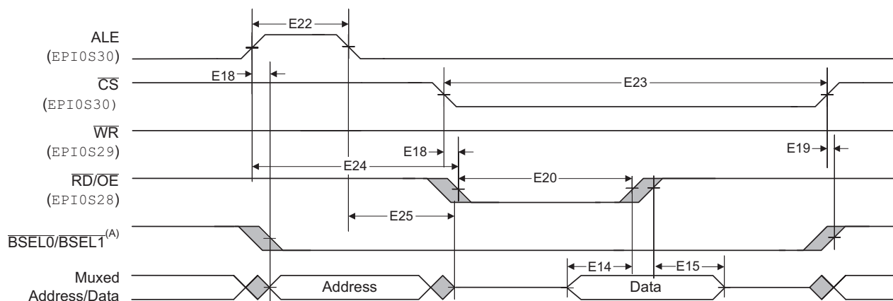
Figure 6-17. Host-Bus 8/16 Mode Muxed Read Timing
