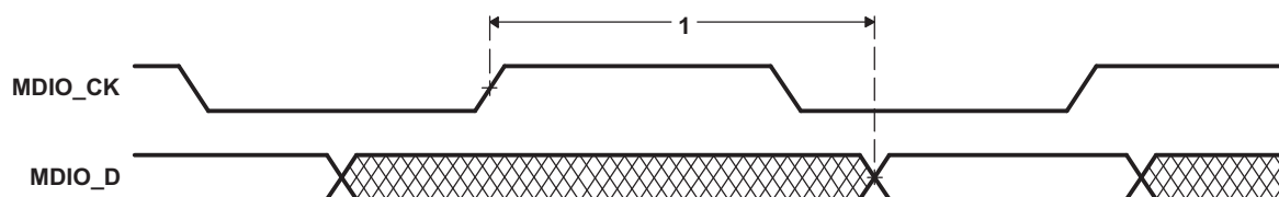
Figure 6-32. MII Serial Management Timing – MDIO as Output
