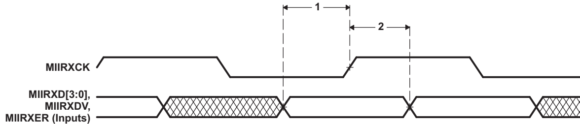
Figure 6-30. 100/10Mb/s MII Receive Timing
