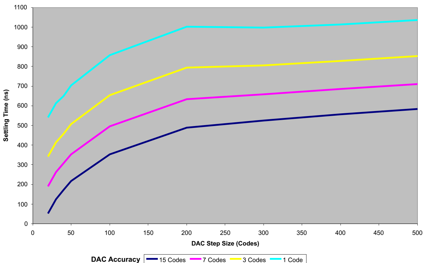
Figure 6-5. DAC Settling Time
