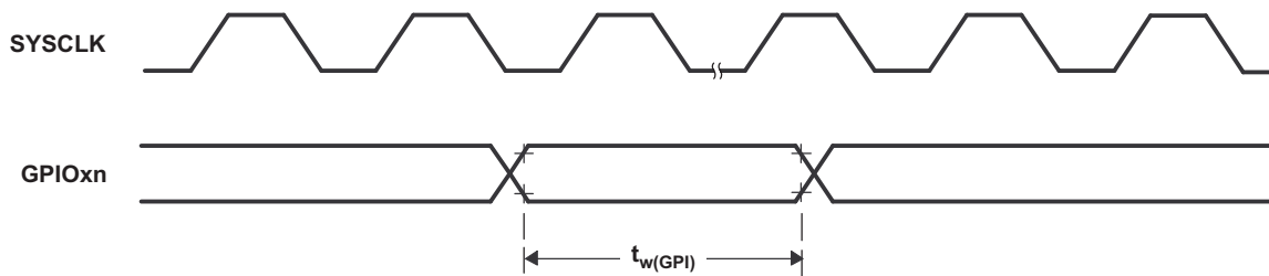
Figure 5-7. General-Purpose Input Timing
