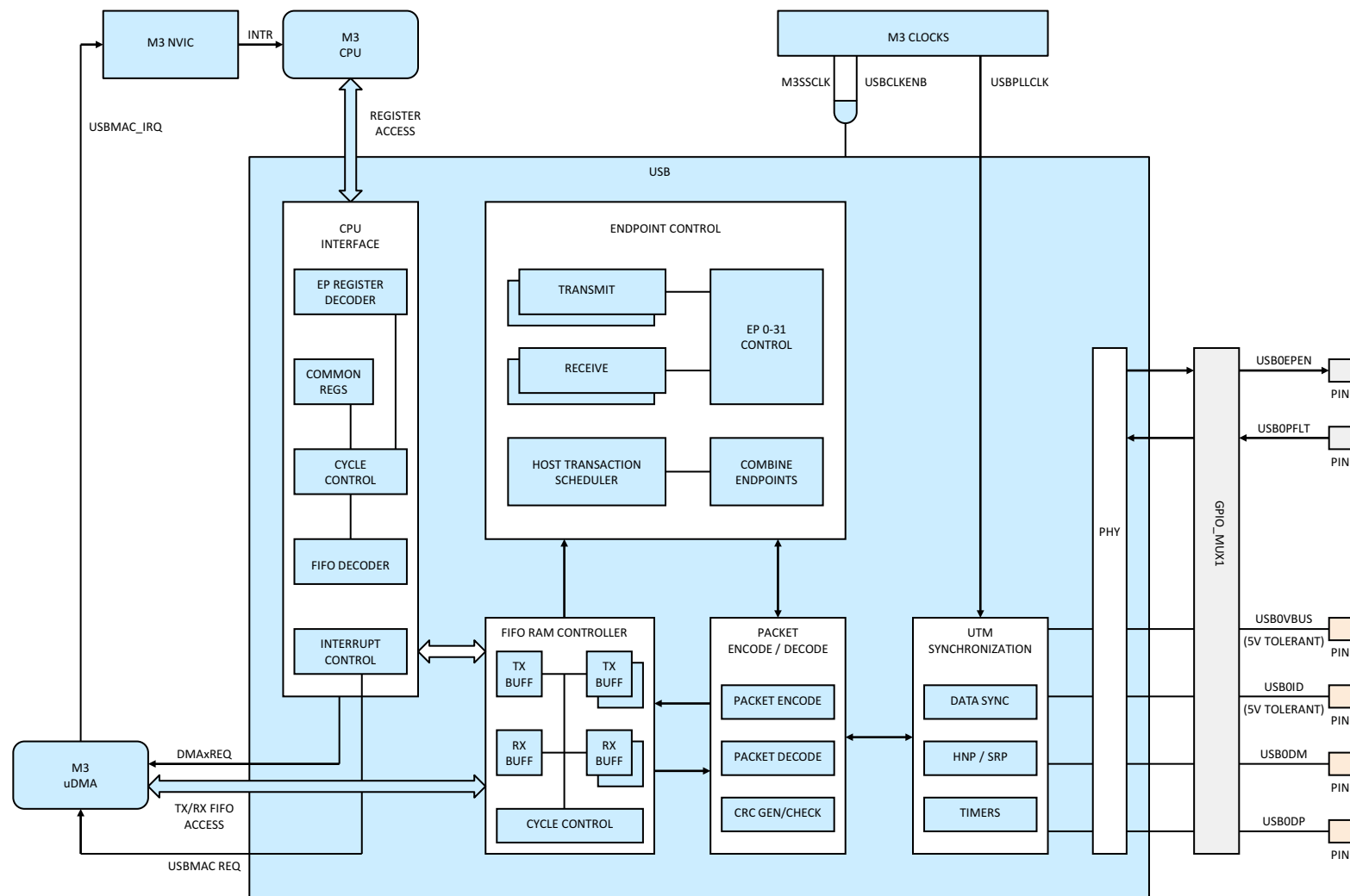
Figure 6-25. USB
