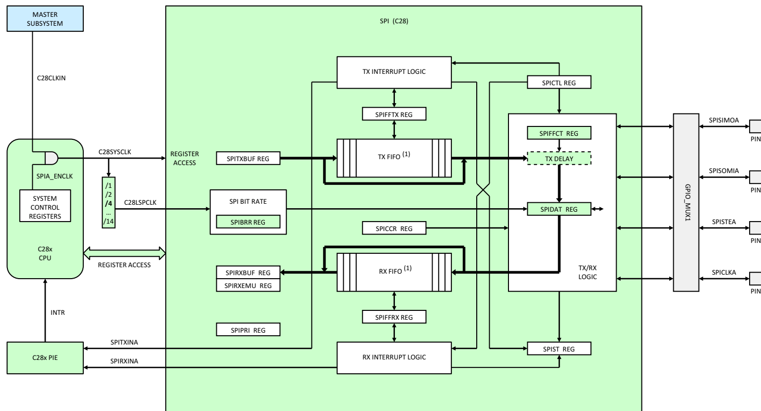
Figure 6-41. SPI (C28x)
