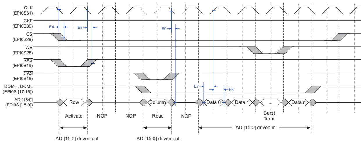
Figure 6-13. SDRAM Read Timing
