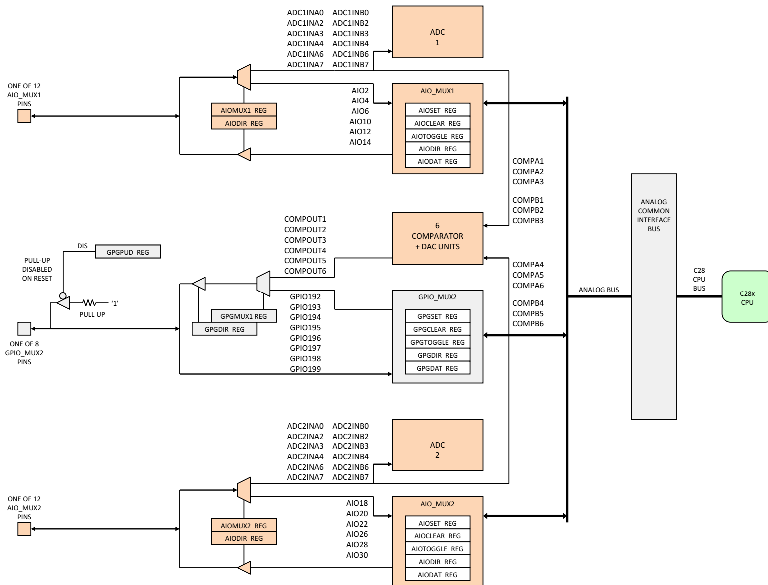
Figure 2-17. Pin Muxing on AIO_MUX1, AIO_MUX2, and GPIO_MUX2
