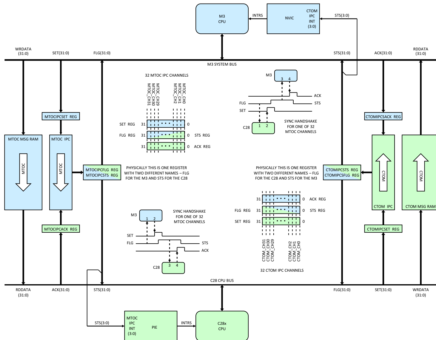
Figure 6-6. Interprocessor Communications (IPC)
