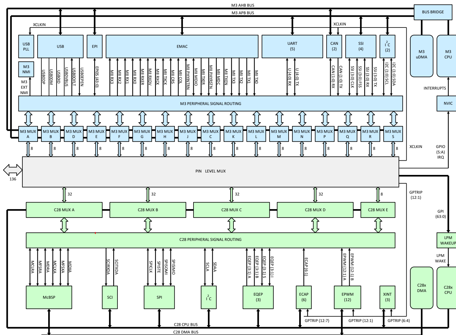
Figure 2-15. GPIO_MUX1 Block
