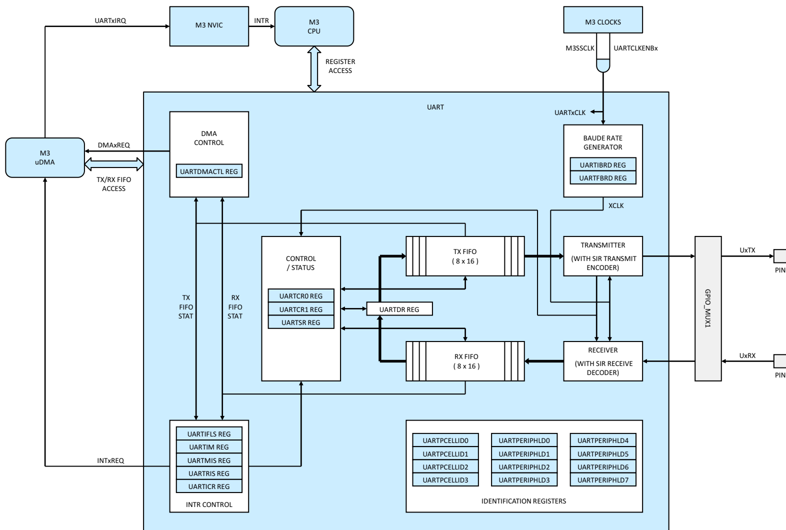
Figure 6-22. UART
