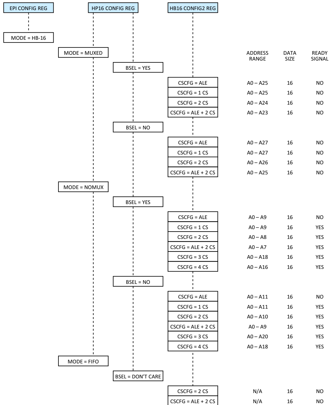
Figure 6-11. EPI 16-Bit Host Bus Mode
