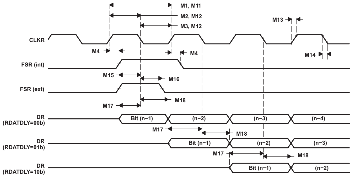
Figure 6-47. McBSP Receive Timing
