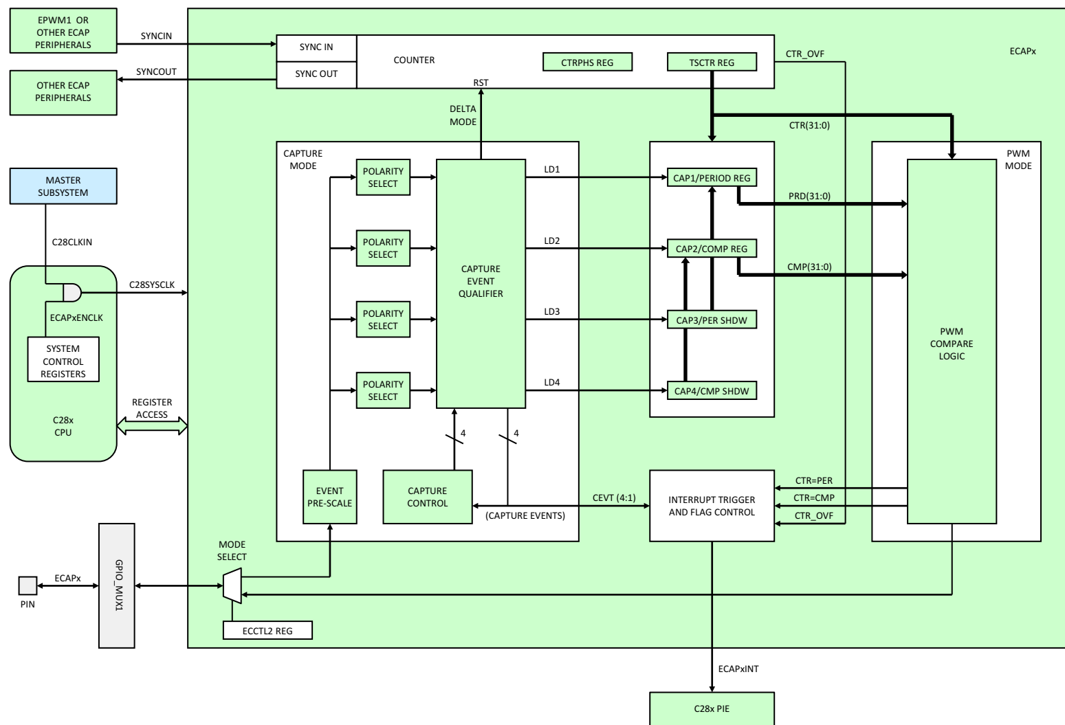
Figure 6-37. eCAP
