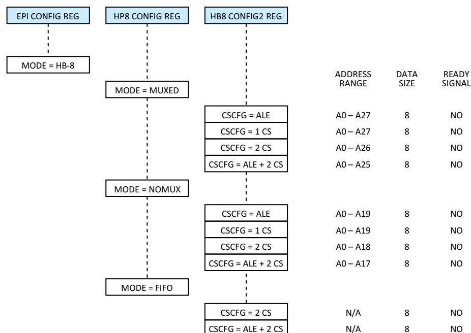
Figure 6-10. EPI 8-Bit Host Bus Mode
