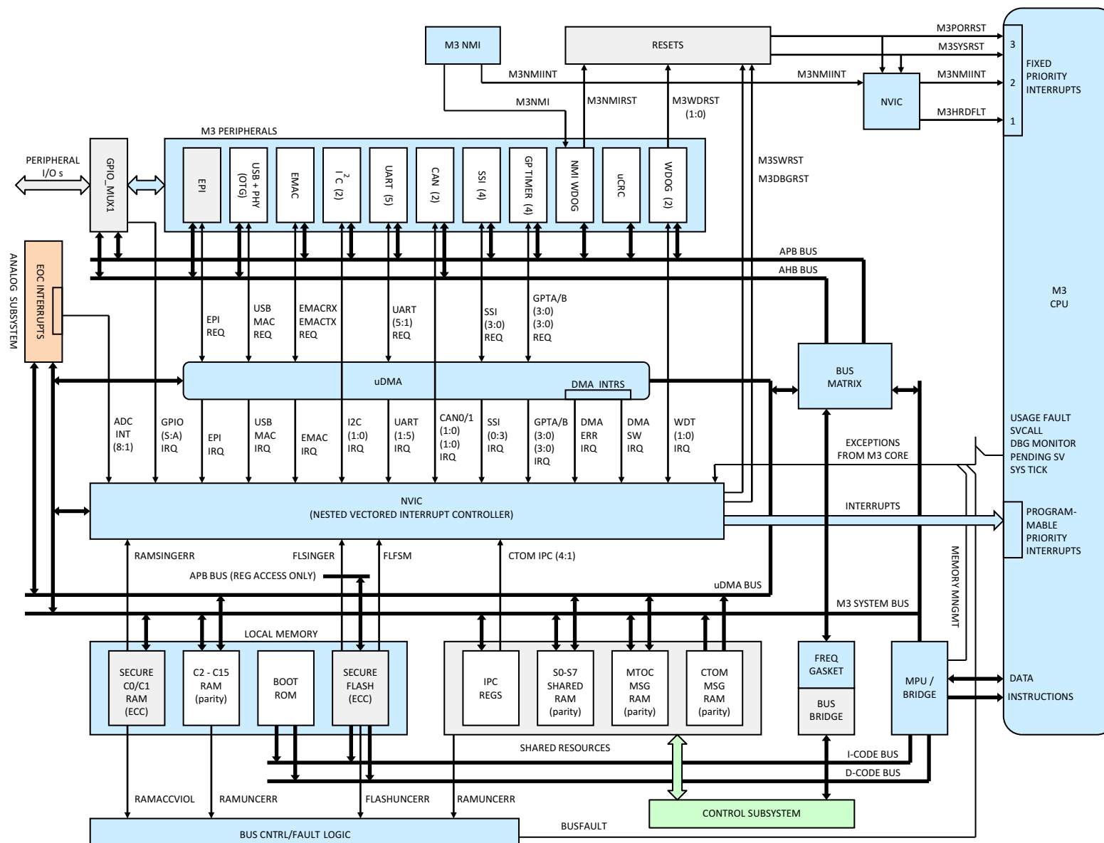
Figure 2-1. Master Subsystem
