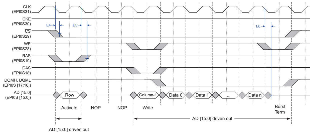
Figure 6-14. SDRAM Write Timing
