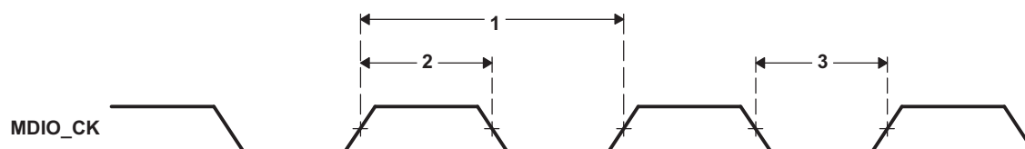
Figure 6-31. MII Serial Management Timing
