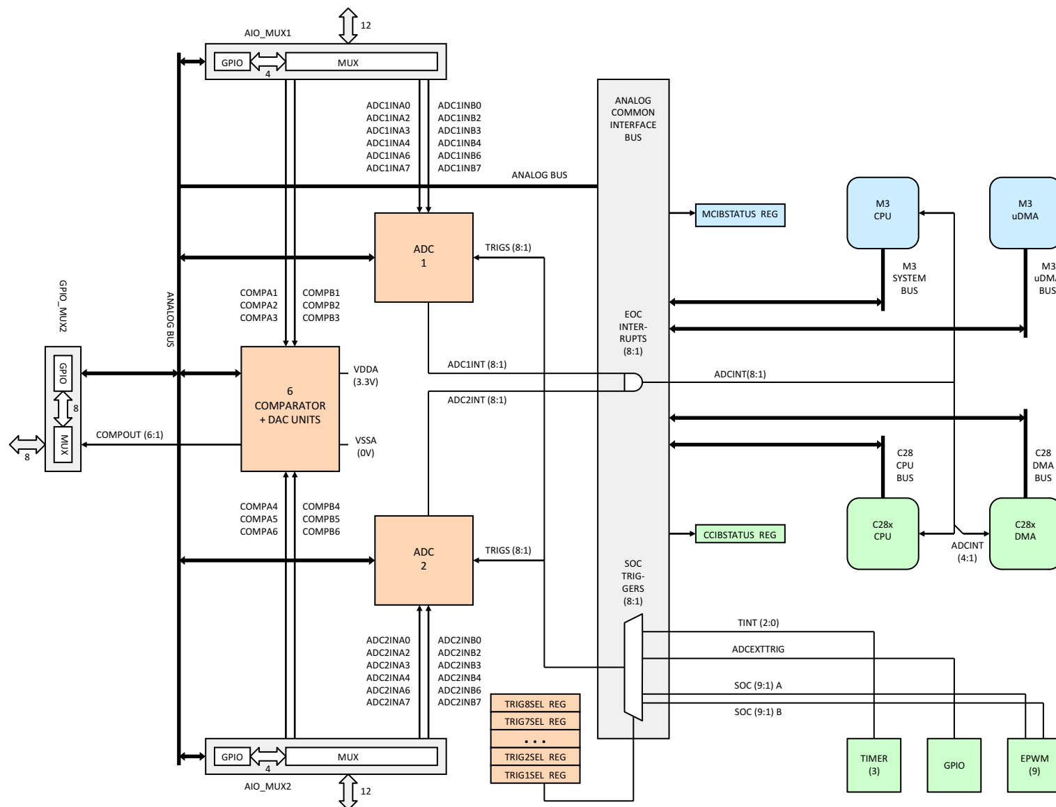
Figure 2-3. Analog Subsystem
