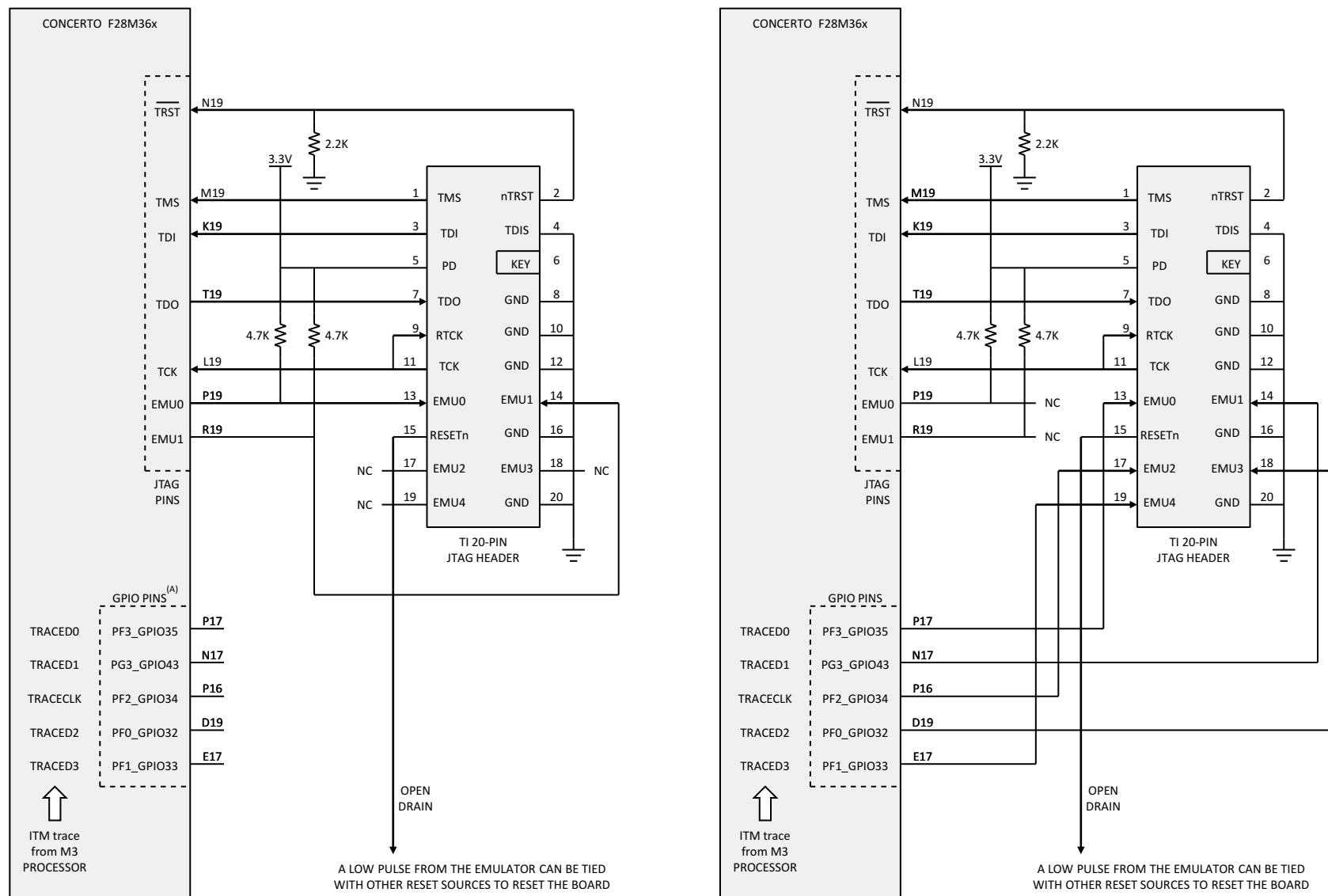
Figure 2-19. Connecting to TI 20-Pin JTAG Emulator Header
