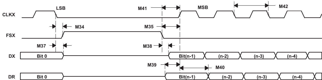
Figure 6-50. McBSP Timing as SPI Master or Slave: CLKSTP = 11b, CLKXP = 0
