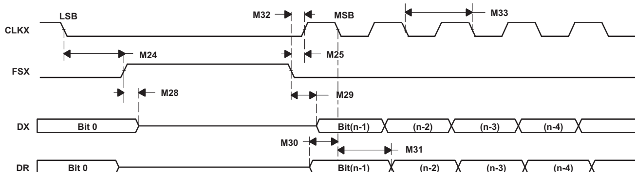
Figure 6-49. McBSP Timing as SPI Master or Slave: CLKSTP = 10b, CLKXP = 0
