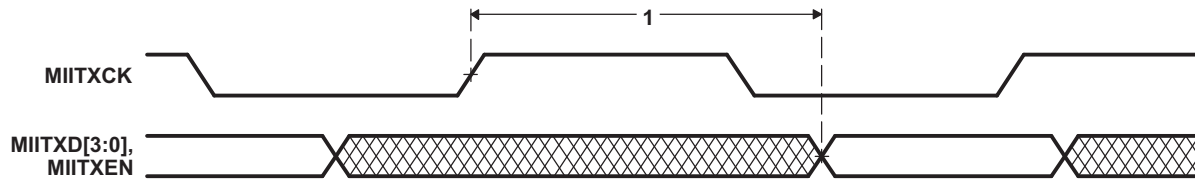
Figure 6-29. 100/10Mb/s MII Transmit Timing
