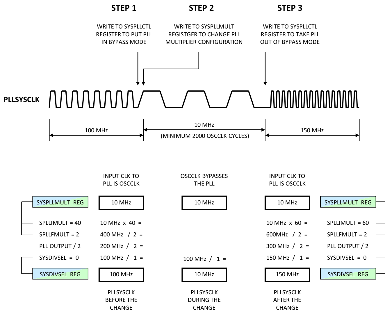
Figure 5-4. Changing the Frequency of the Main PLL
