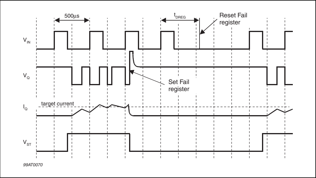
Figure 14. Recirculation error
