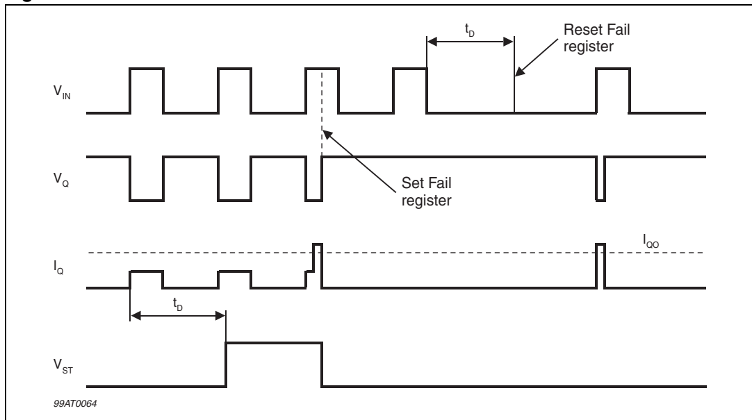
Figure 8. Current overload
