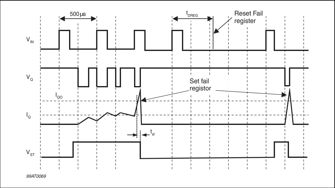
Figure 14. Recirculation error
