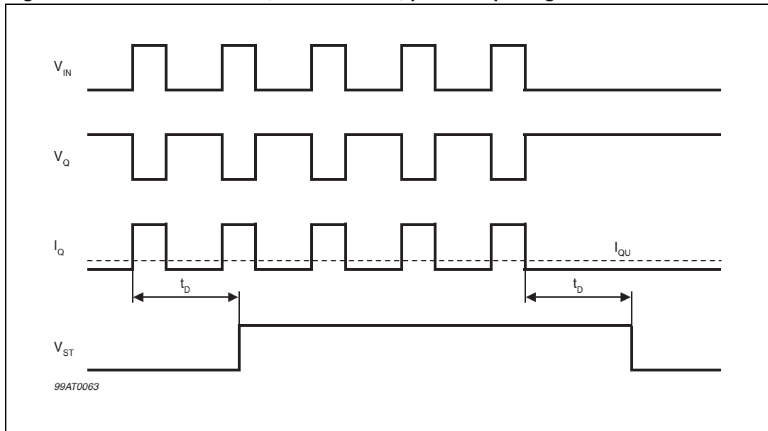
Figure 8. Current overload
