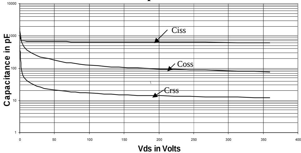
IXZ210N50L Capacitance verses Vds
