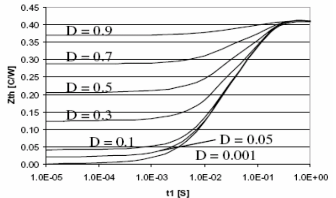
IXZ210N50L Thermal Response
