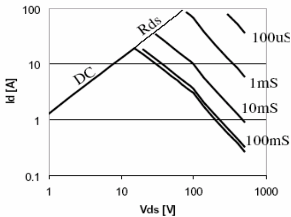
IXZ210N50L Safe Operating Area
