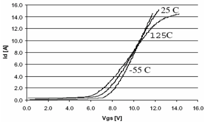
IXZ210N50L Id vs Temp
