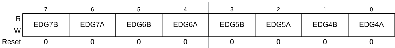
Figure 7-13. Timer Control Register 3 (TCTL3)
