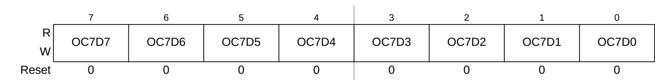
Figure 7-6. Output Compare 7 Data Register (OC7D)
