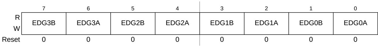
Figure 7-14. Timer Control Register 4 (TCTL4)
