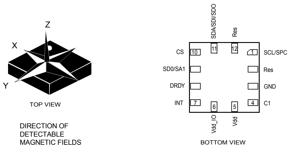
Figure 2. Pin description
