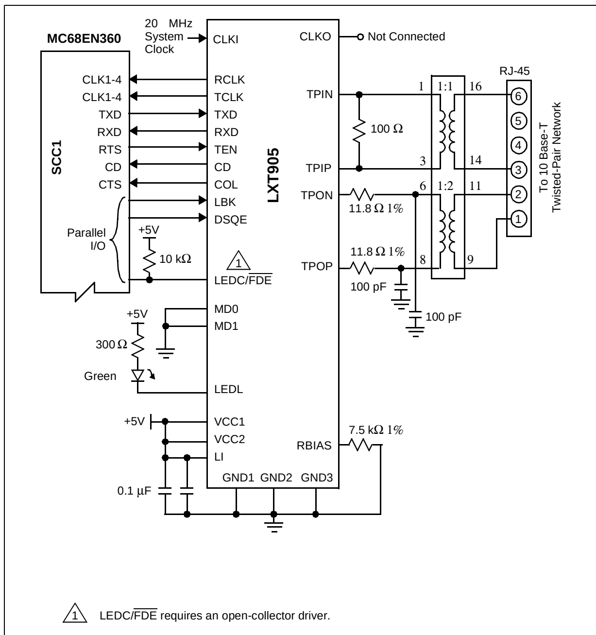
Figure 10. LXT905/MC68EN360 Interface for Full-Duplex 10BASE-T (Mode 1)
