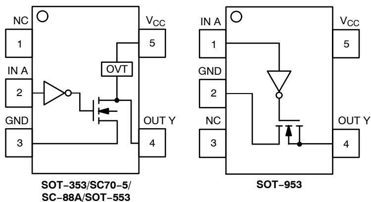
Figure 1. Pinout
