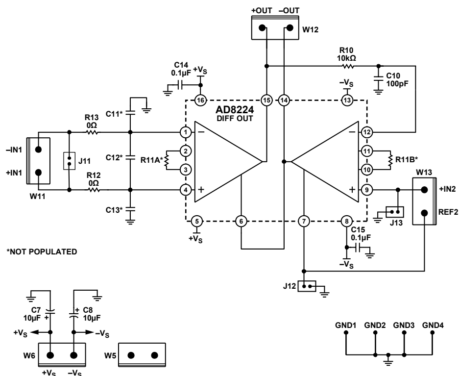
Figure 3. AD8224 Evaluation Board Schematic—AD8224 Differential Output
