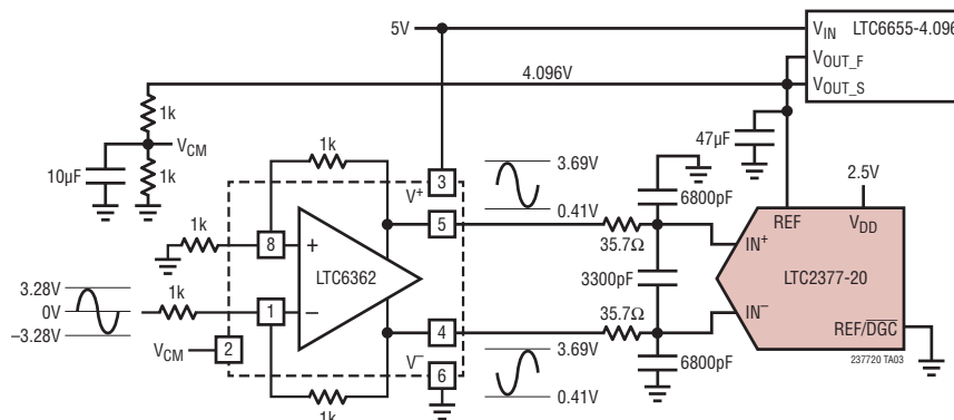
LTC6362 Configured to Accept a \pm 3.28\text{V} Input Signal While Running from a Single 5V Supply with Digital Gain Compression Enabled in the LTC2377-20
